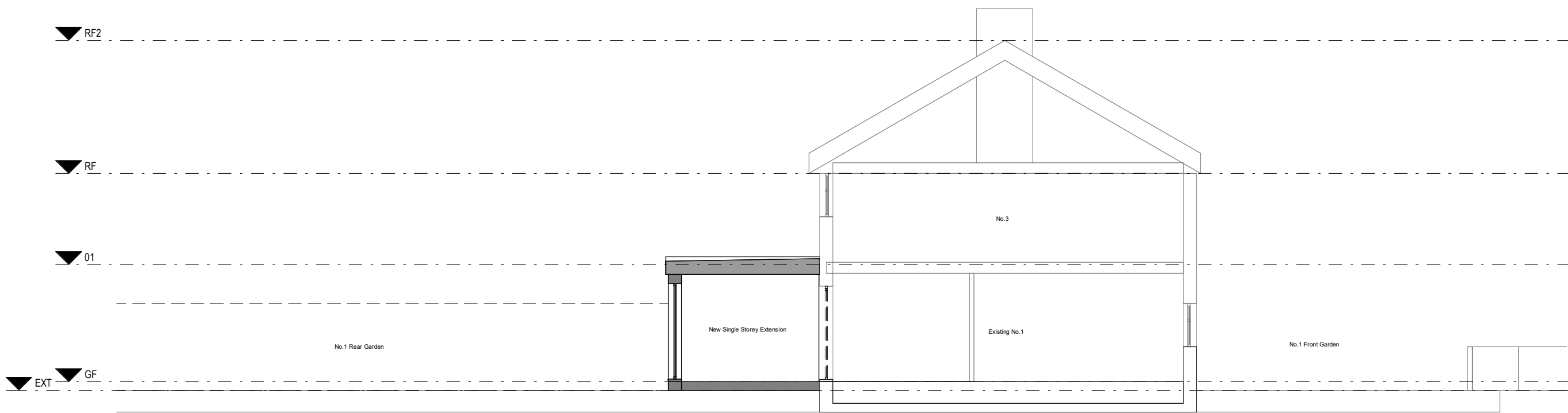
1 East - West Section 07-0010 1 : 100
