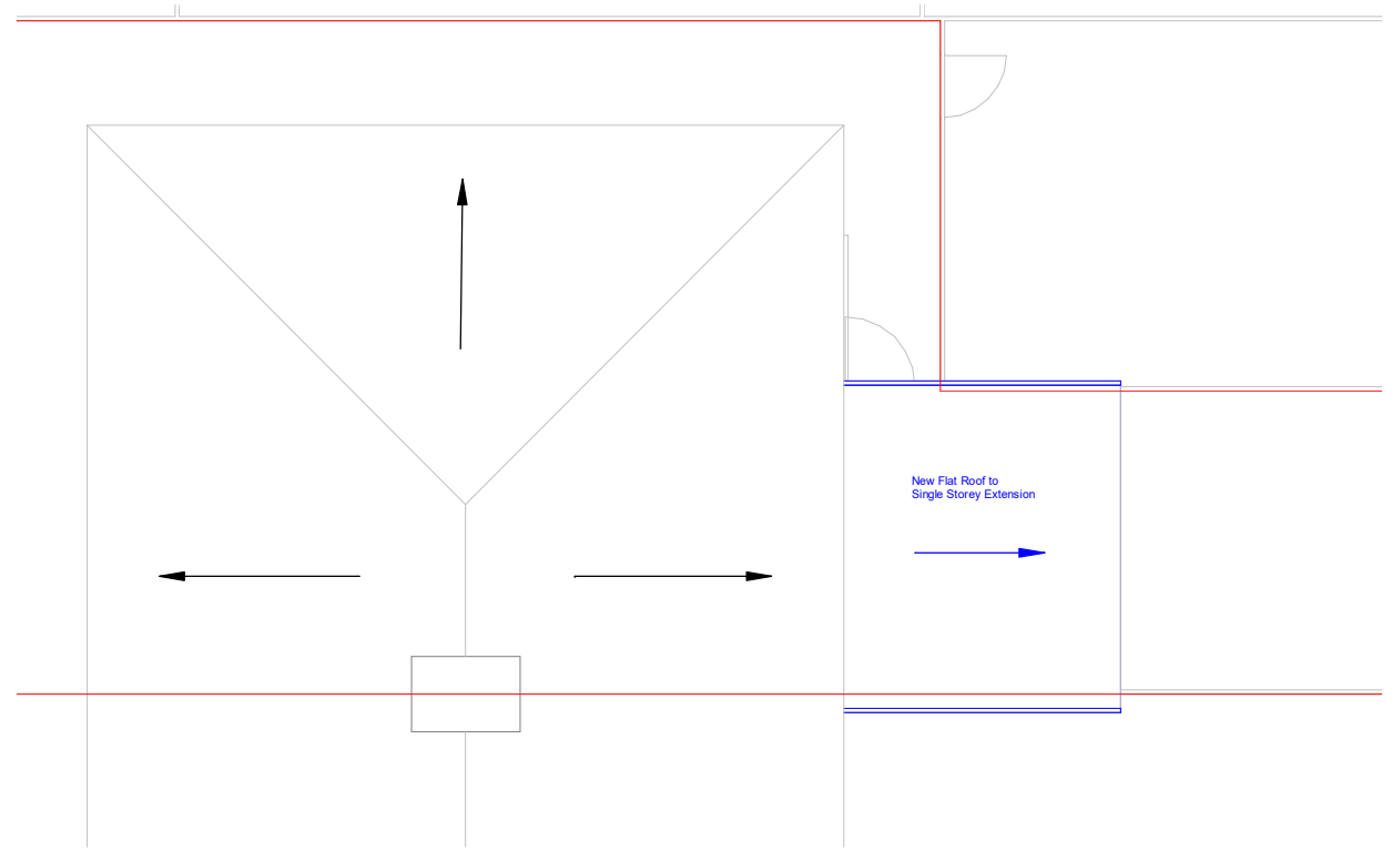
2 Proposed Roof Plan 04-0010 1: 100
