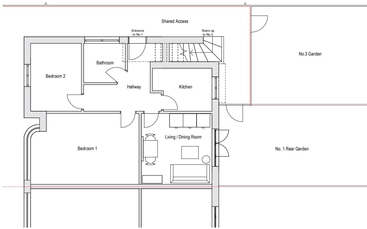
1 Existing Ground Floor Plan 04-0010 1: 100
