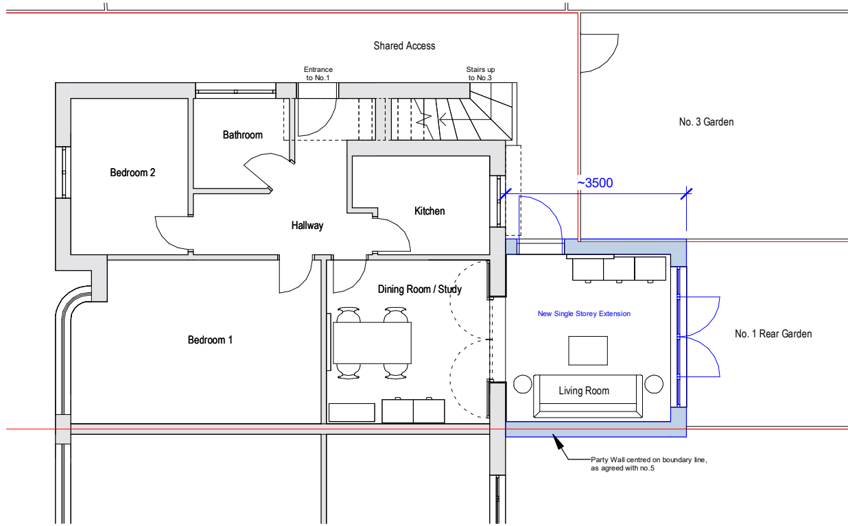
3 Proposed Ground Floor Plan 04-0010 1: 100
