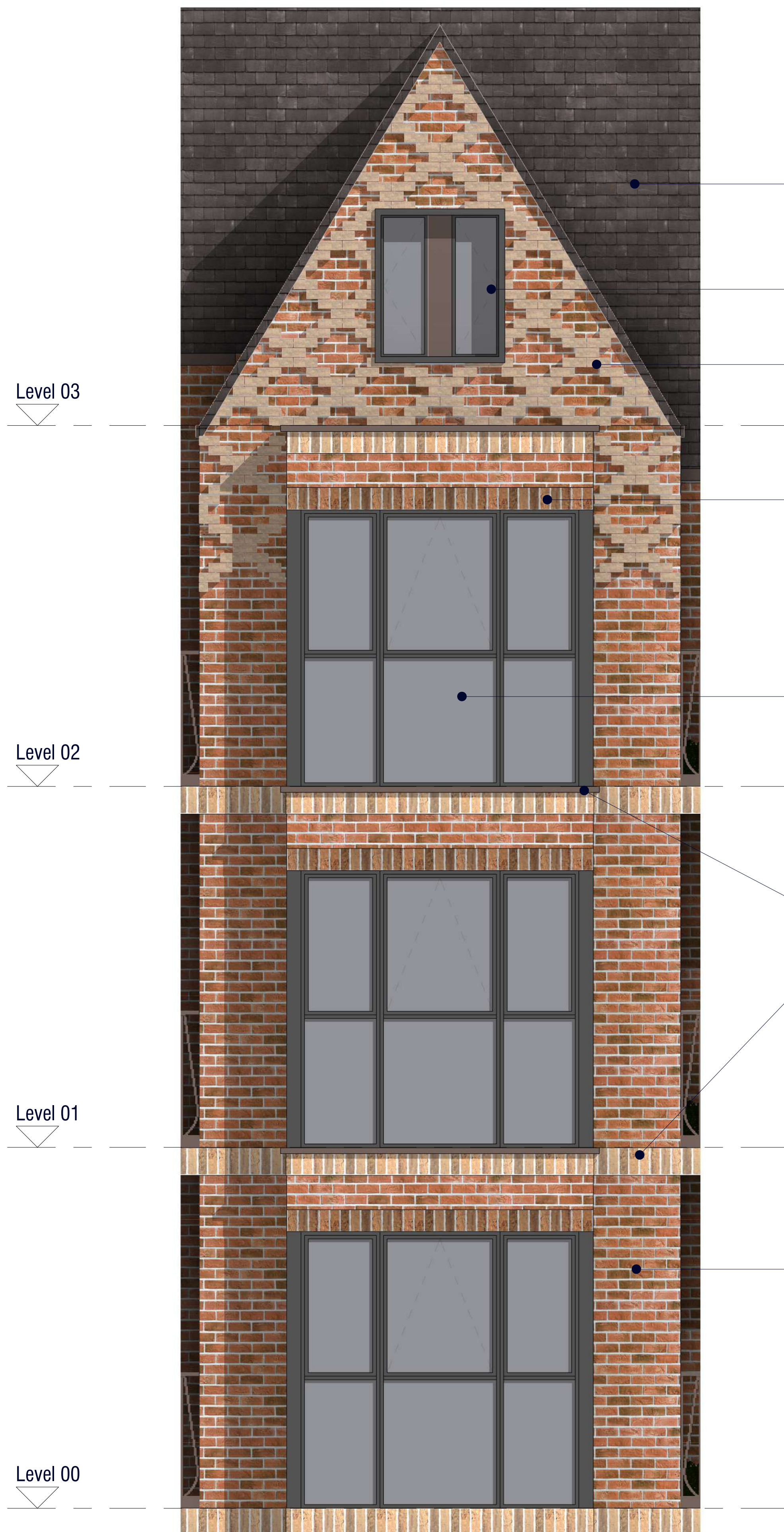
1 Typical Gable Elevation 1 : 25
