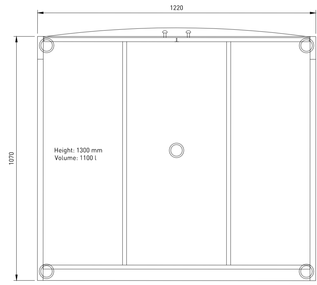
02 1100L BIN DIMENSIONS 1:10
