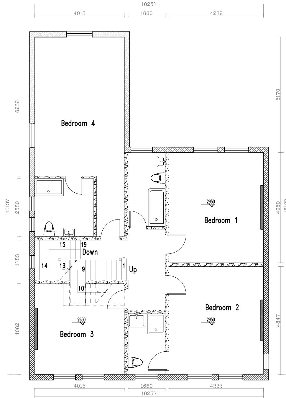
Existing First Floor Plan 1-100 @ A3
