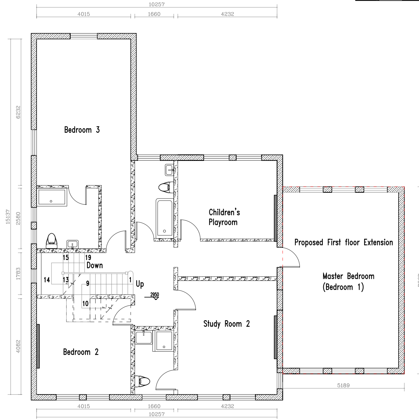
Proposed Floor Plan 1-100 @ A3
