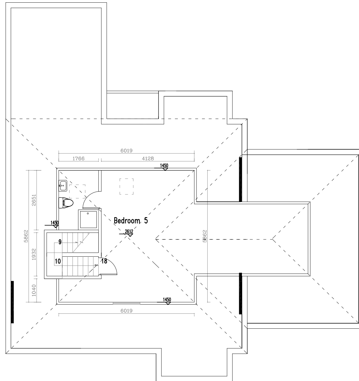
Proposed second Floor Plan 1-100 @ A3
