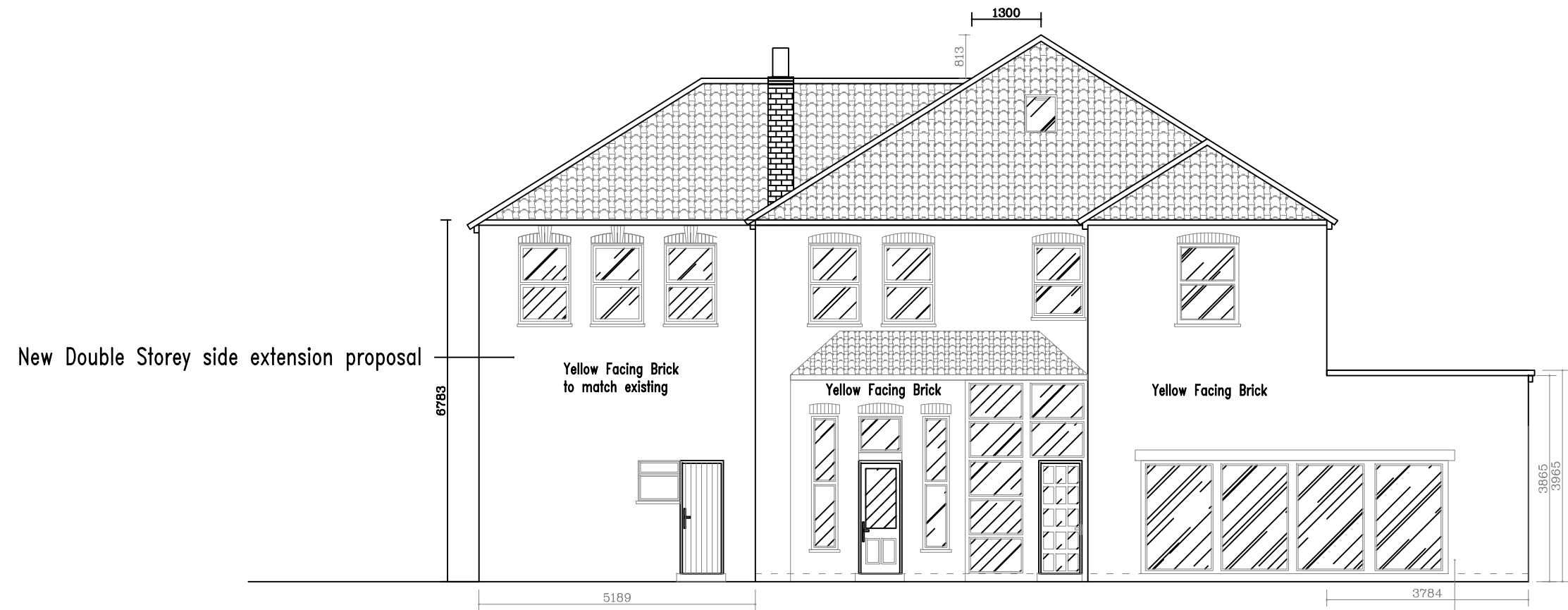
Proposed Rear Elevation 1-100 @ A3
