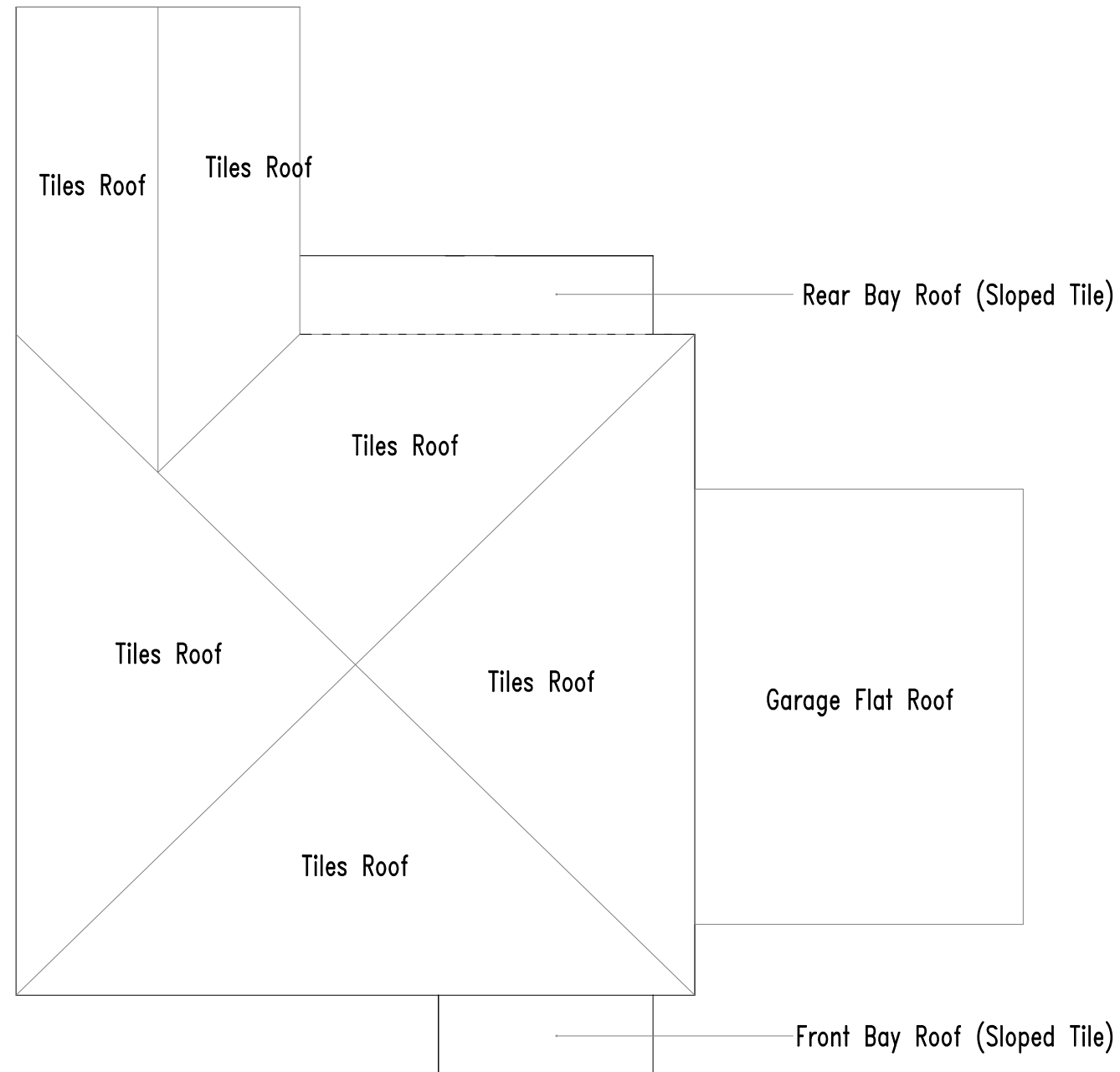
Existing Roof Plan 1-100 @ A3
