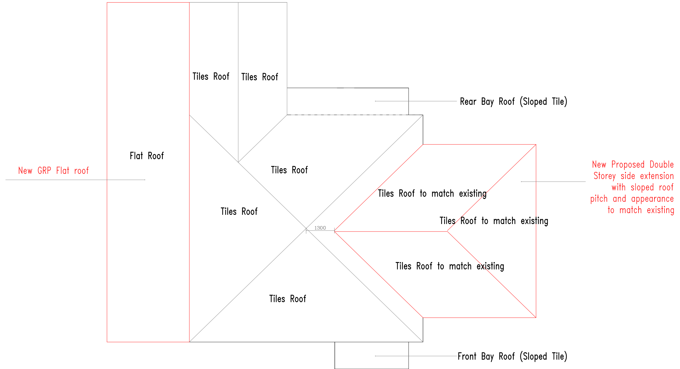
Proposed Roof Plan 1-100 @ A3
