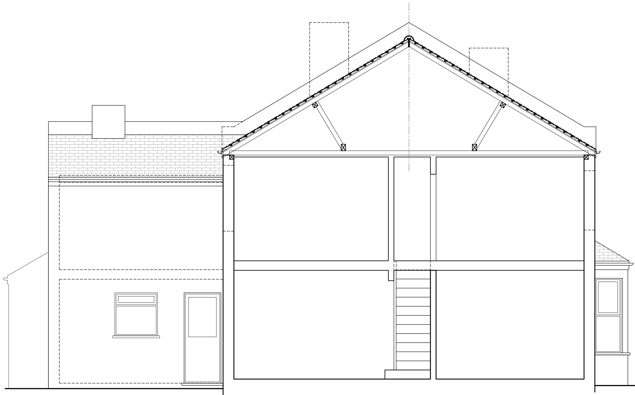
Existing Section Scale 1/50@A3
