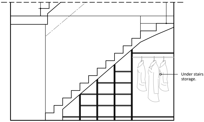
Proposed section through stairs Scale 1/50@A3
