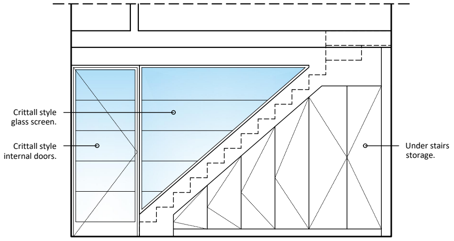
Interior elevation - Stairs's wall from the dining area Scale 1/50@A3
