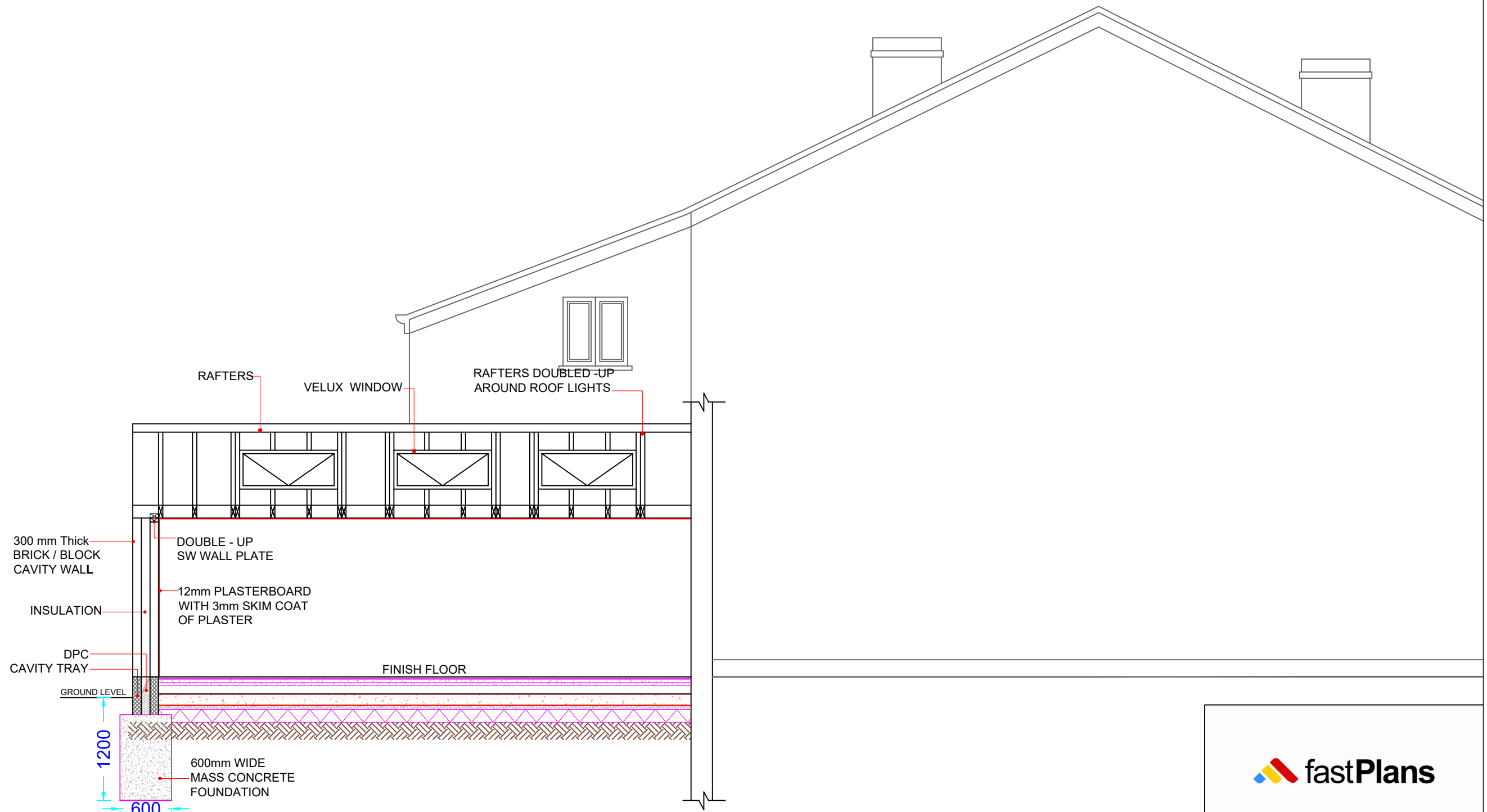
PROPOSED SECTION AA SCALE 1:50
