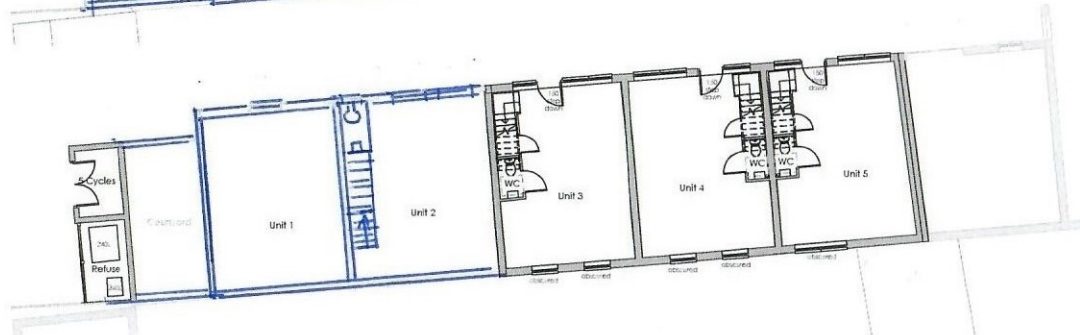
Ground Floor 1:100
