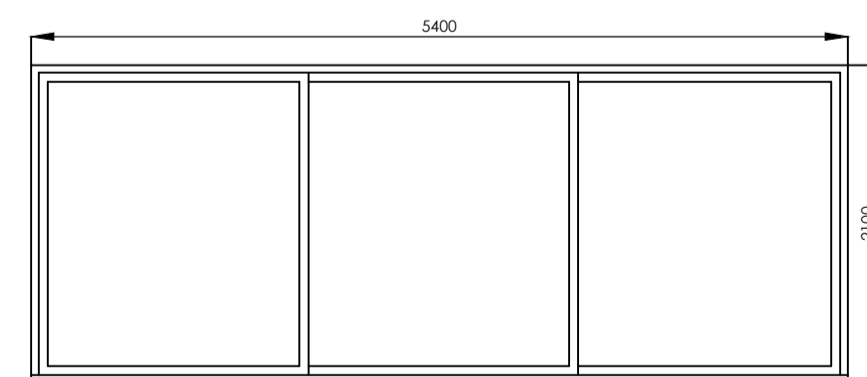
DOOR/WINDOW DETAILS
