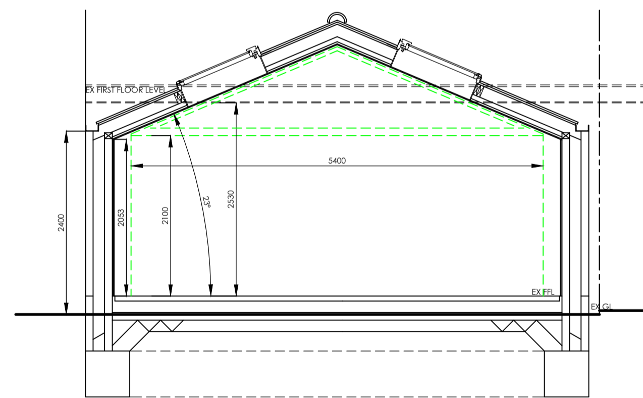
PROPOSED SECTION 1:50
