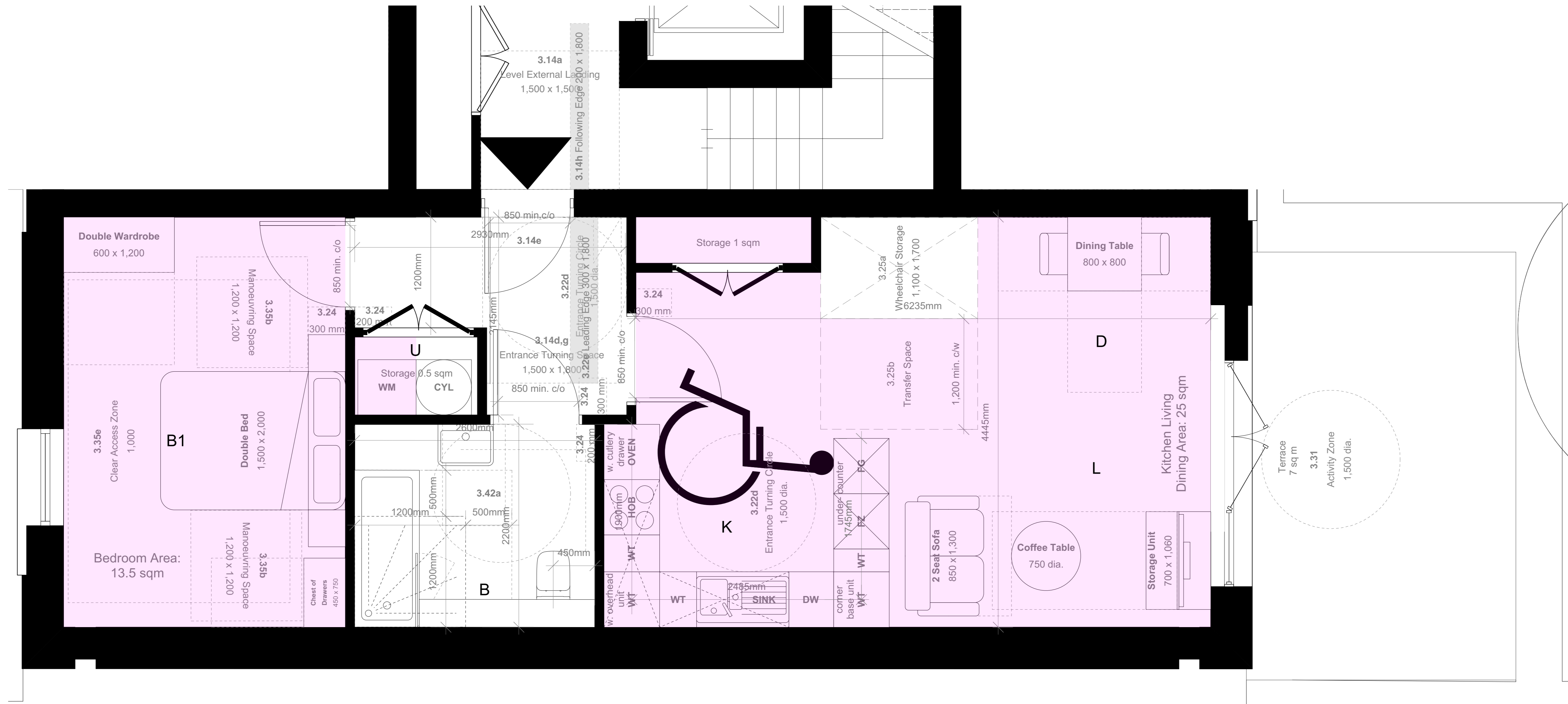
Typical M4(3) Accessible 1 Bed Apartment
