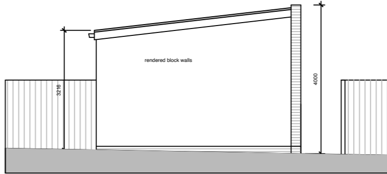
SOUTH SIDE ELEVATION
