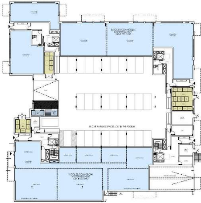
NOCCE1: GROUND FLOOR PLAN
