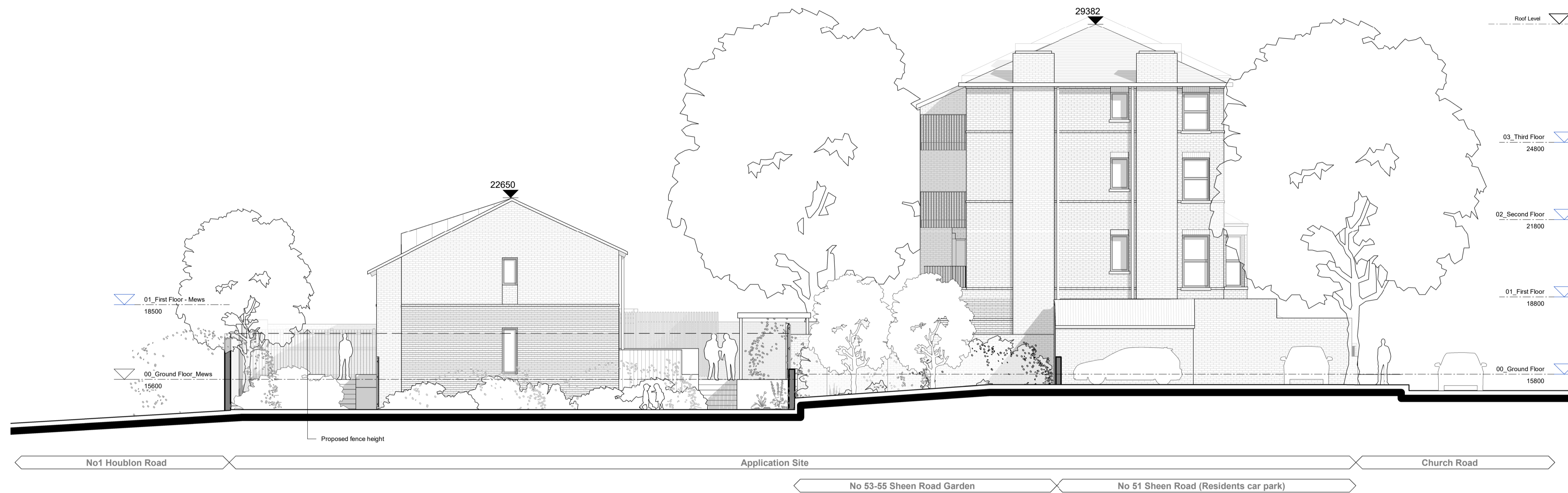
1 Proposed North Elevation 1 : 100
