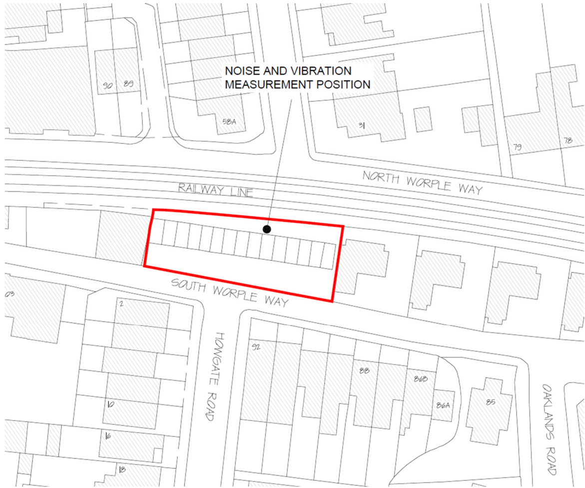
Figure 1 : Location Plan showing measurement position for noise and vibration
