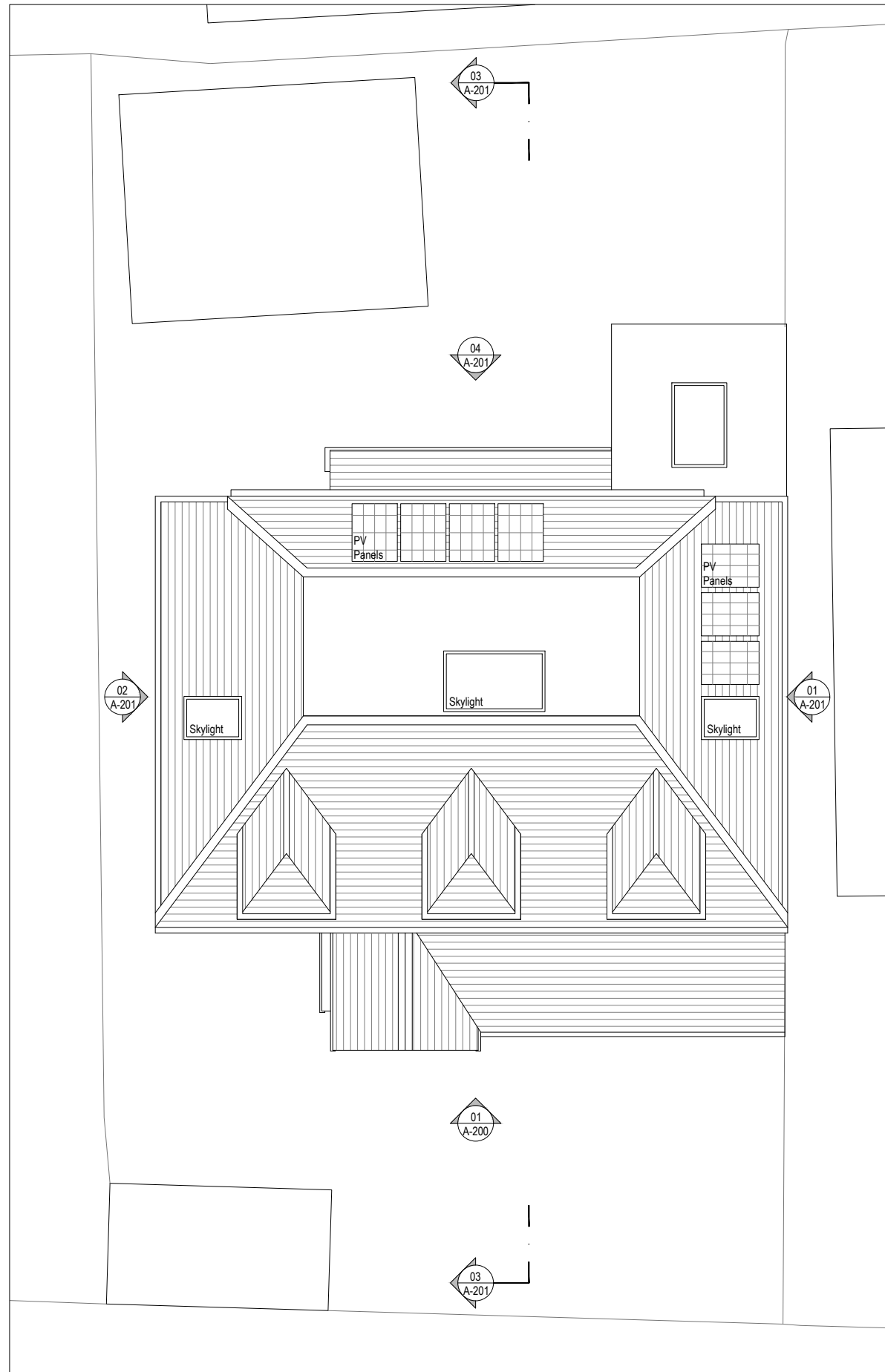
01 Proposed Roof Plan 1:100 @ A3
