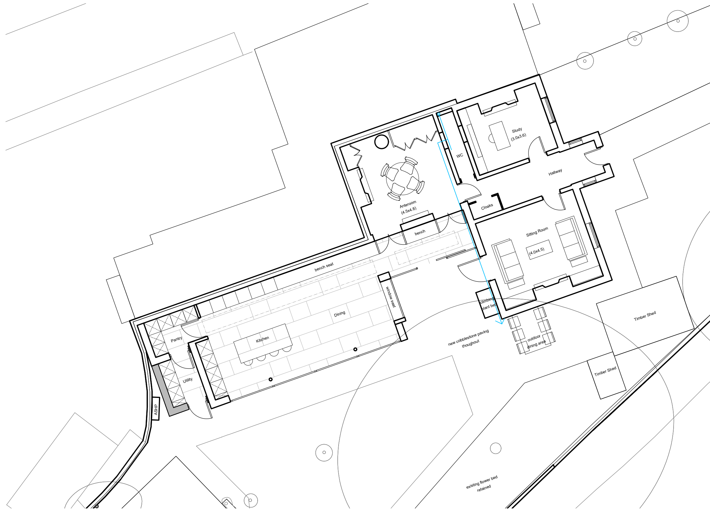
1 Proposed Ground Floor Plan Scale: 1:100
