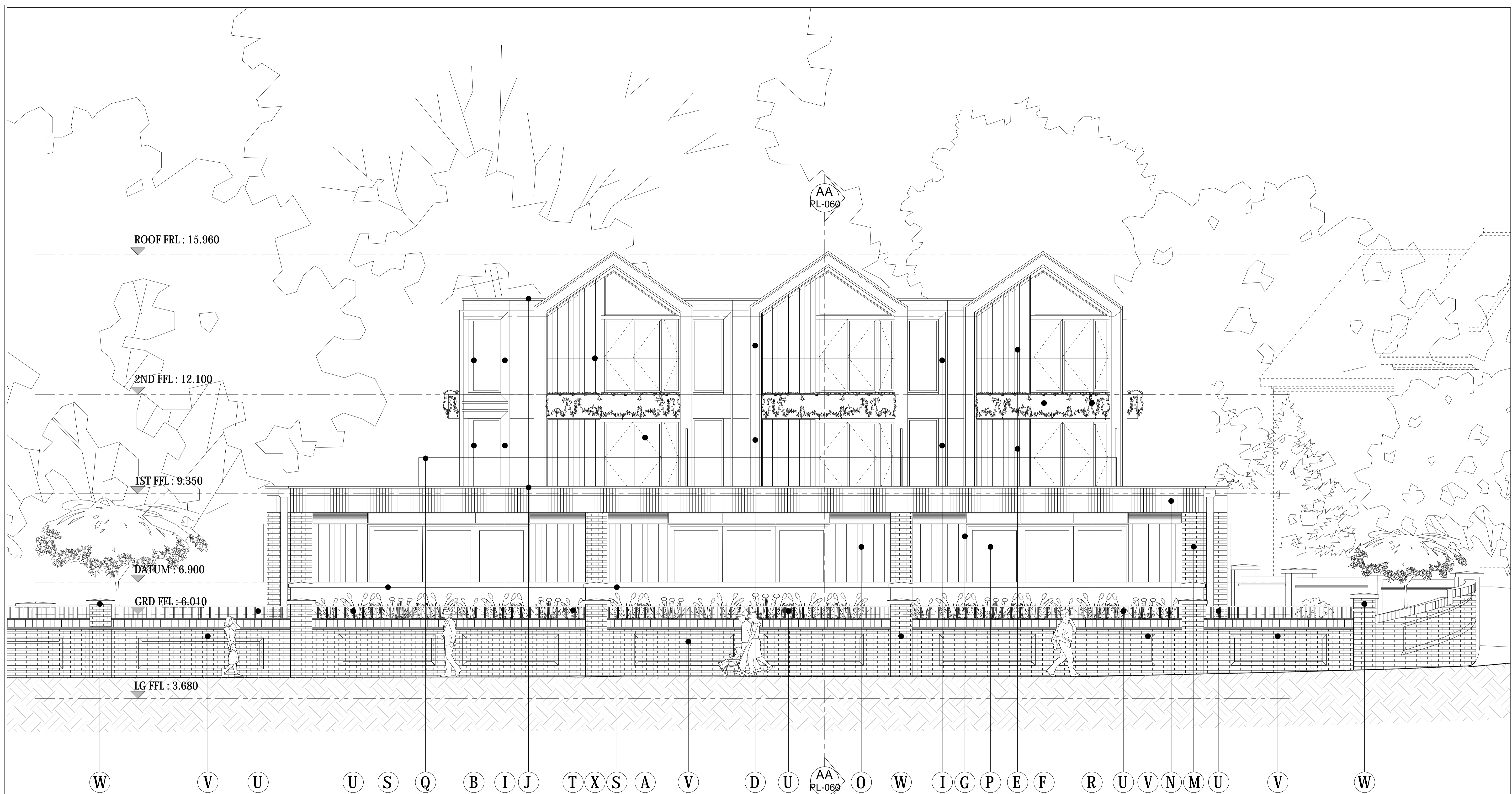
Proposed North Elevation Scale @ 1:50
