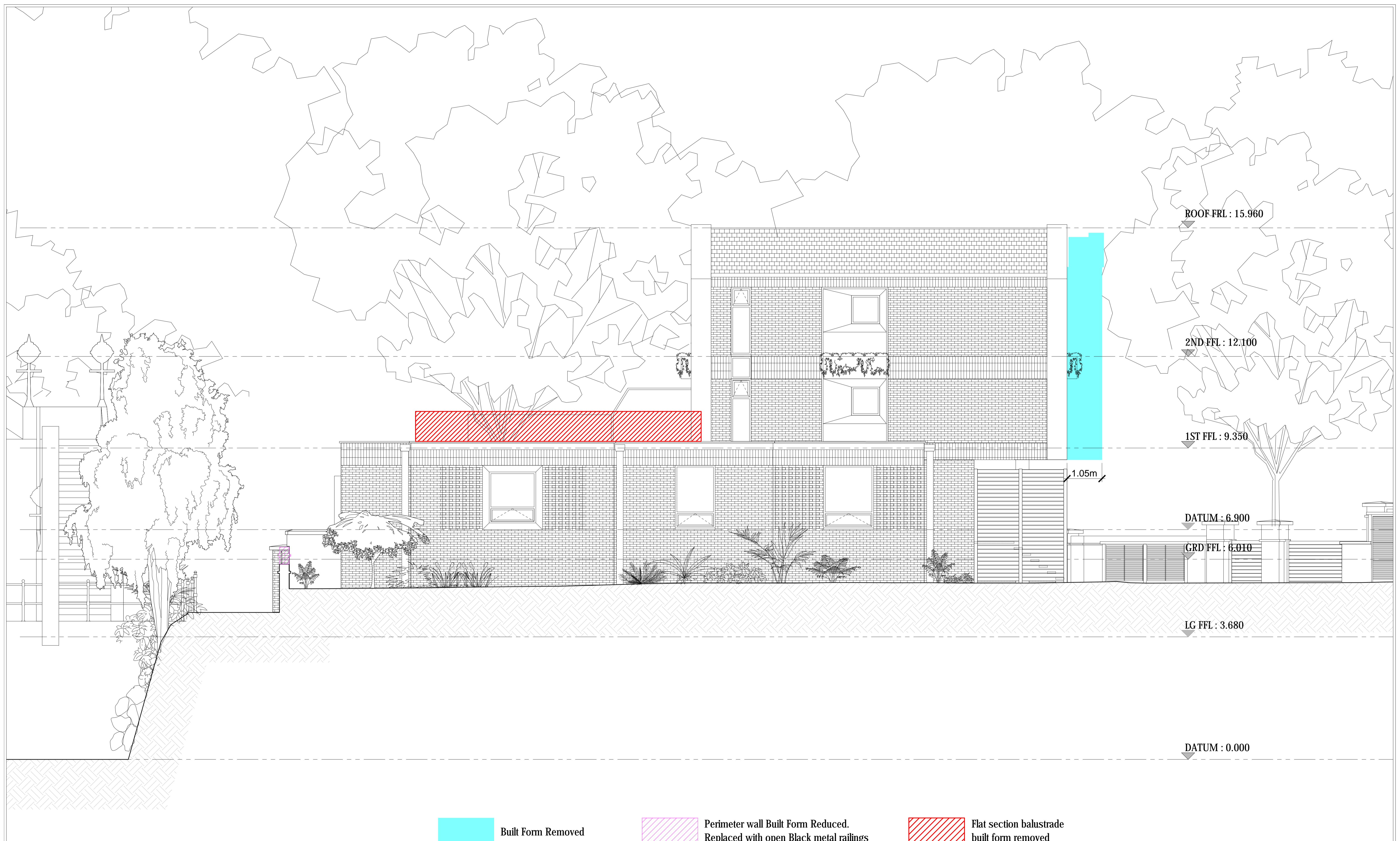
Proposed West Elevation Scale @ 1:50
