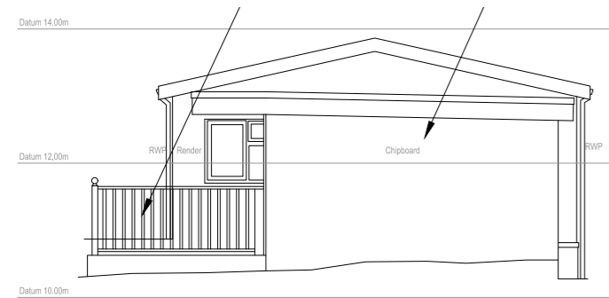
10 ELEVATION 10 SCALE - 1:50 @ A1
