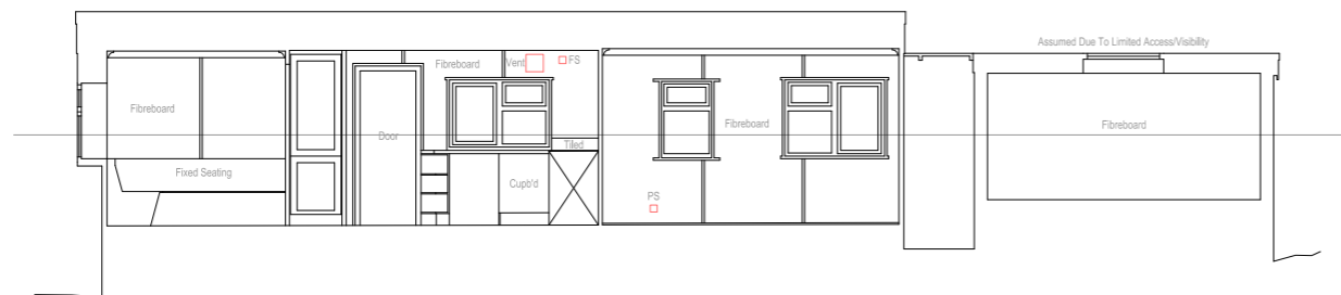
SC3 SECTION 3 SCALE - 1:50 @ A1
