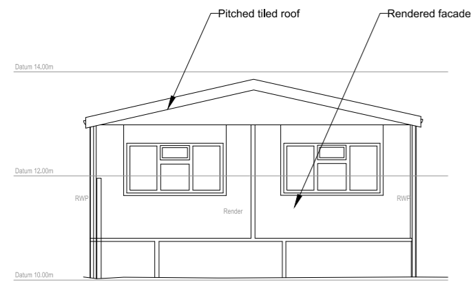
10 ELEVATION 10 SCALE - 1:50 @ A1
