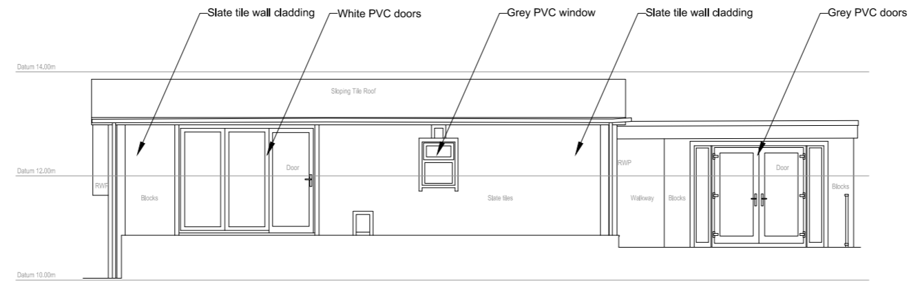
11 ELEVATION 11 SCALE - 1:50 @ A1
