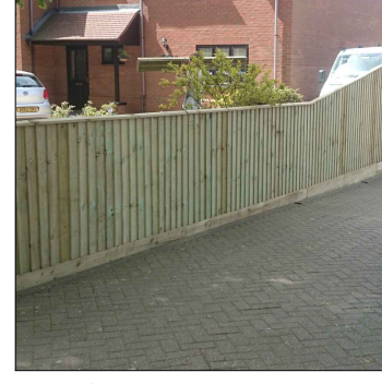
Example 9. Rear Terraces: Timber close board fences, 1200mm high with capping rail and gravel boards
