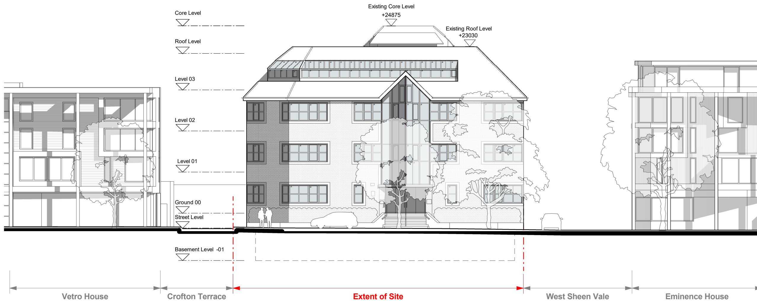
1 Existing North Elevation 1 : 200
