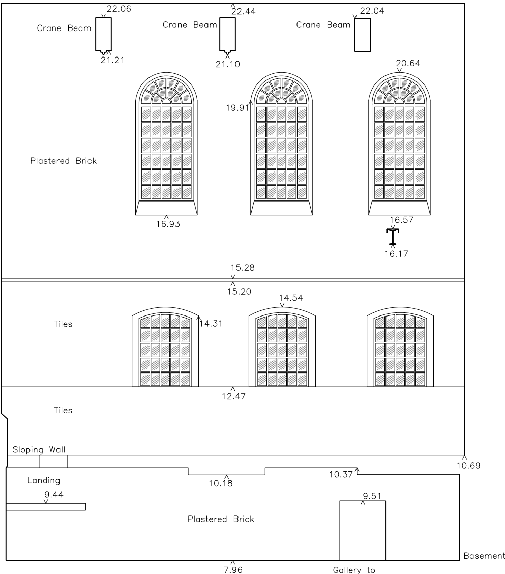
7.00m AOD SCALE 1:100 RUSTON & WARD - Pumphouse Elevation 2
