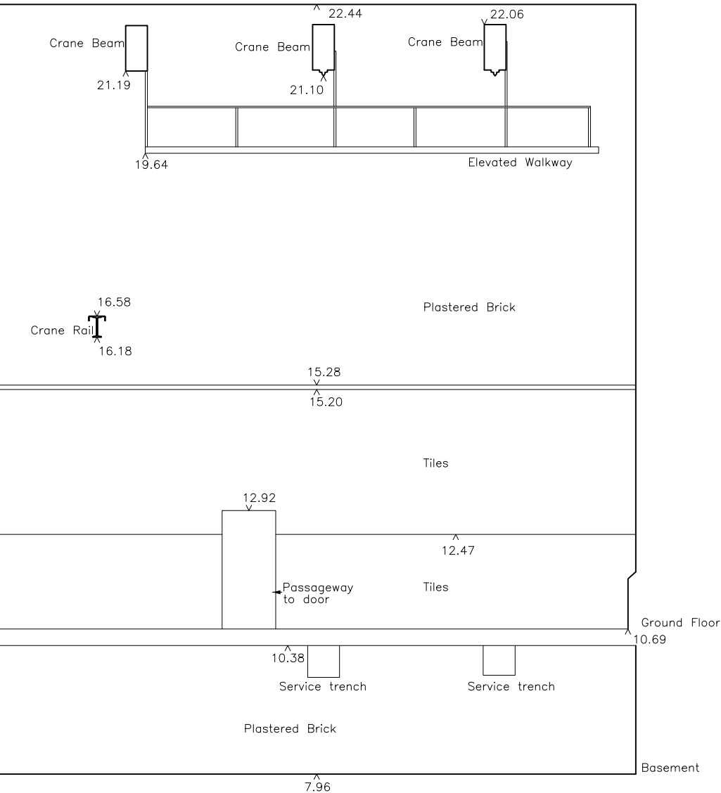
7.00m AOD SCALE 1:100 RUSTON & WARD - Pumphouse Elevation 4
