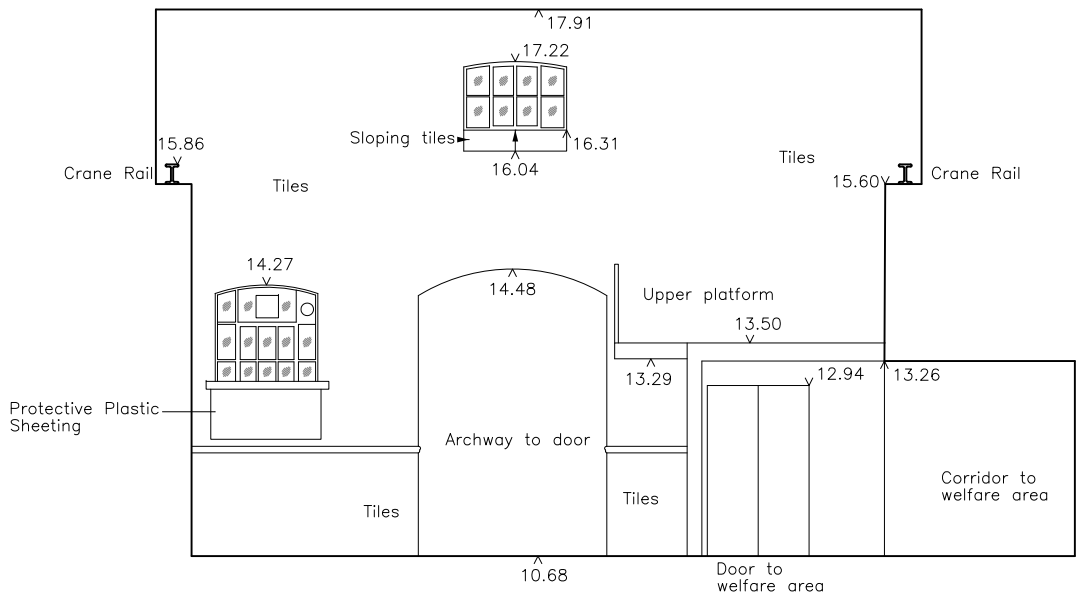
7.00m AOD SCALE 1:100 RUSTON & WARD - Workshop Elevation 1
