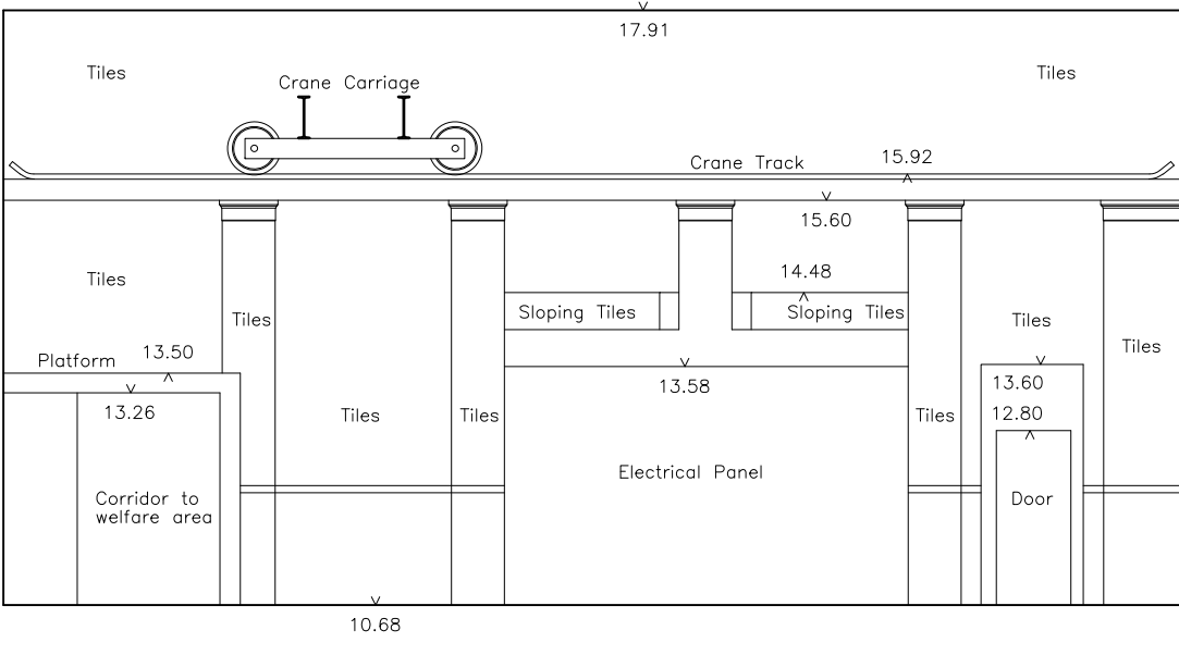
7.00m AOD SCALE 1:100 RUSTON & WARD - Workshop Elevation 2
