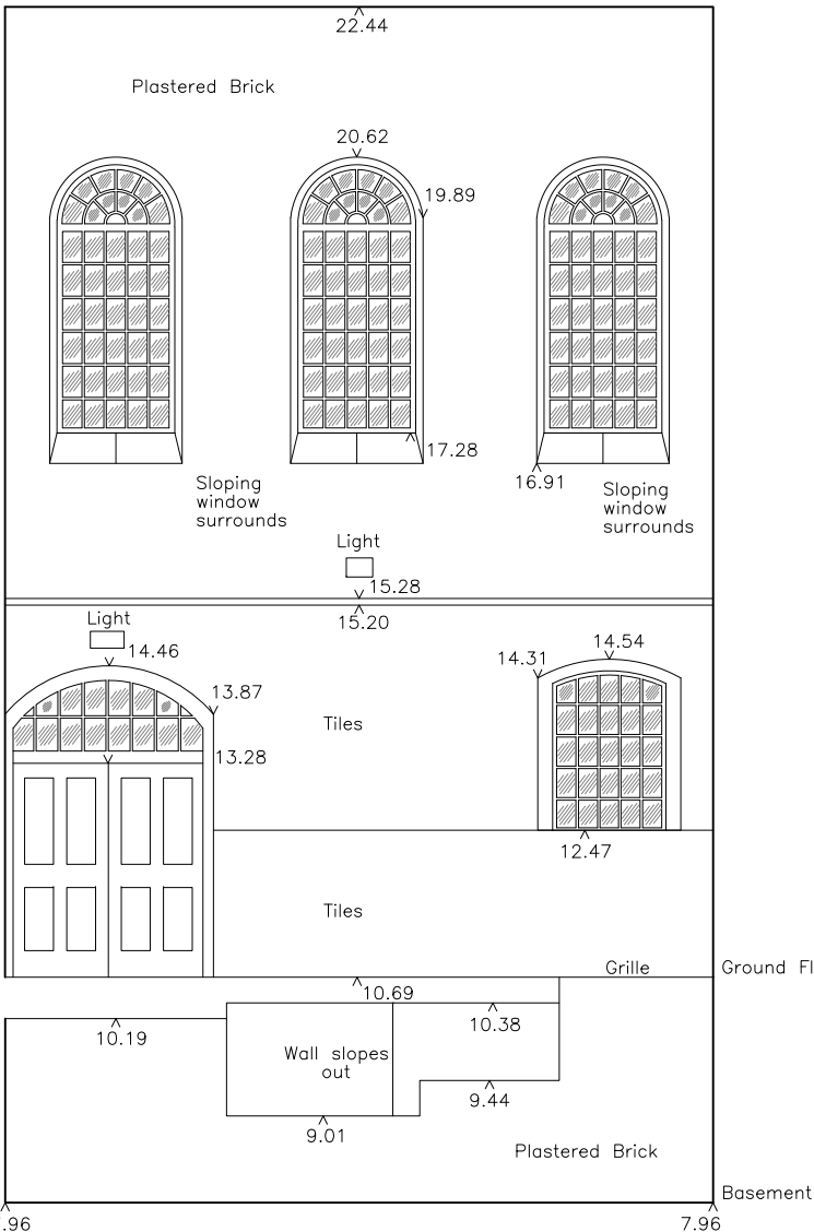
7.00m AOD SCALE 1:100 RUSTON & WARD - Pumphouse Elevation 3
