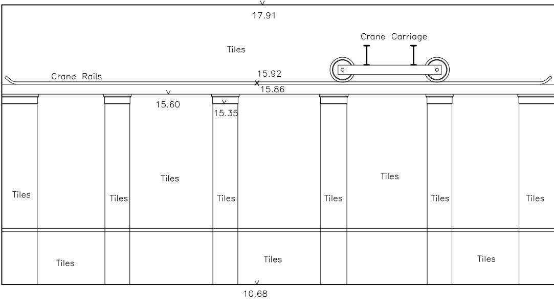
7.00m AOD SCALE 1:100 RUSTON & WARD - Workshop Elevation 4
