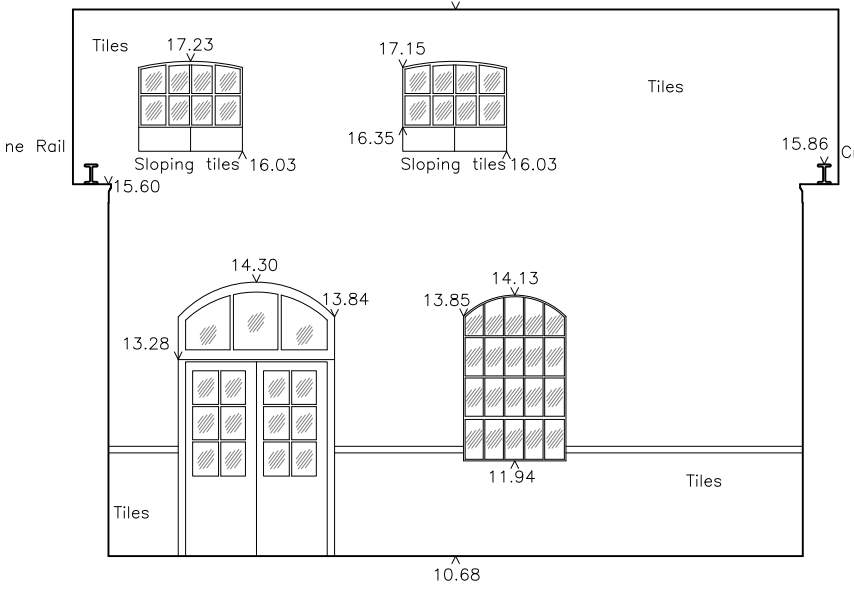
7.00m AOD SCALE 1:100 RUSTON & WARD - Workshop Elevation 3
