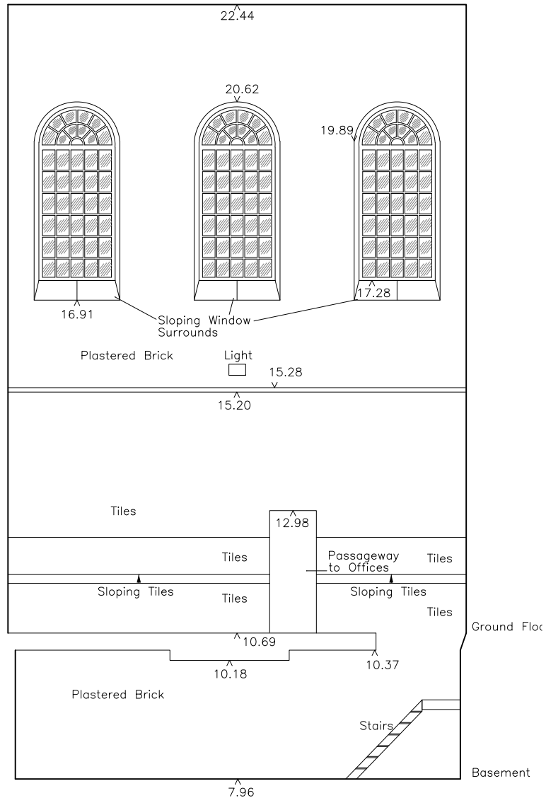
7.00m AOD SCALE 1:100 RUSTON & WARD - Pumphouse Elevation 1
