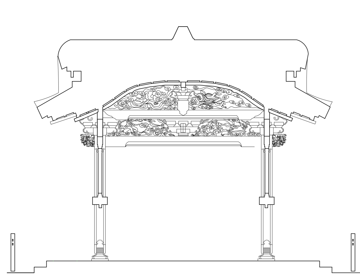
SECTION E-E
