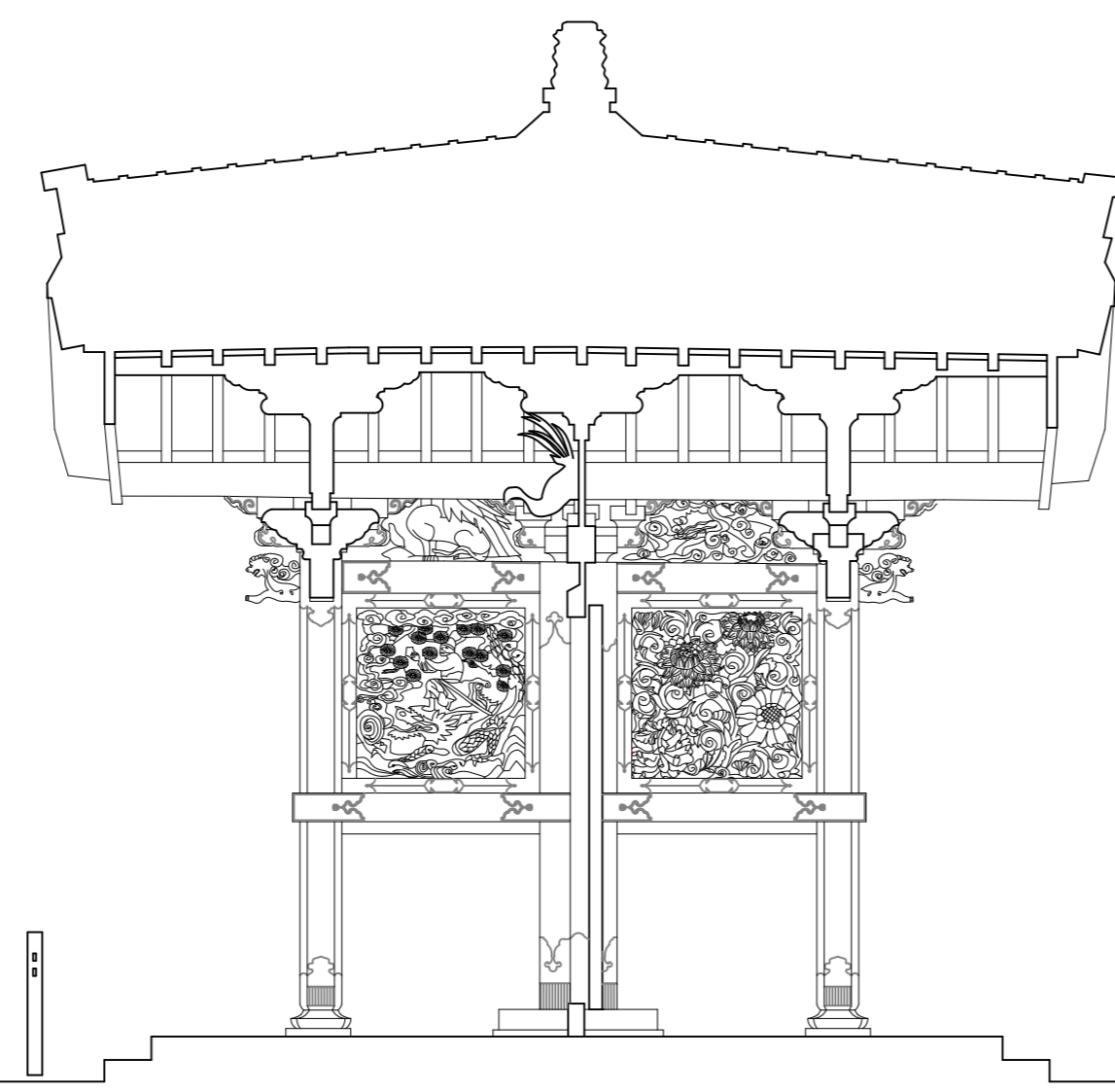
SECTION B-B
