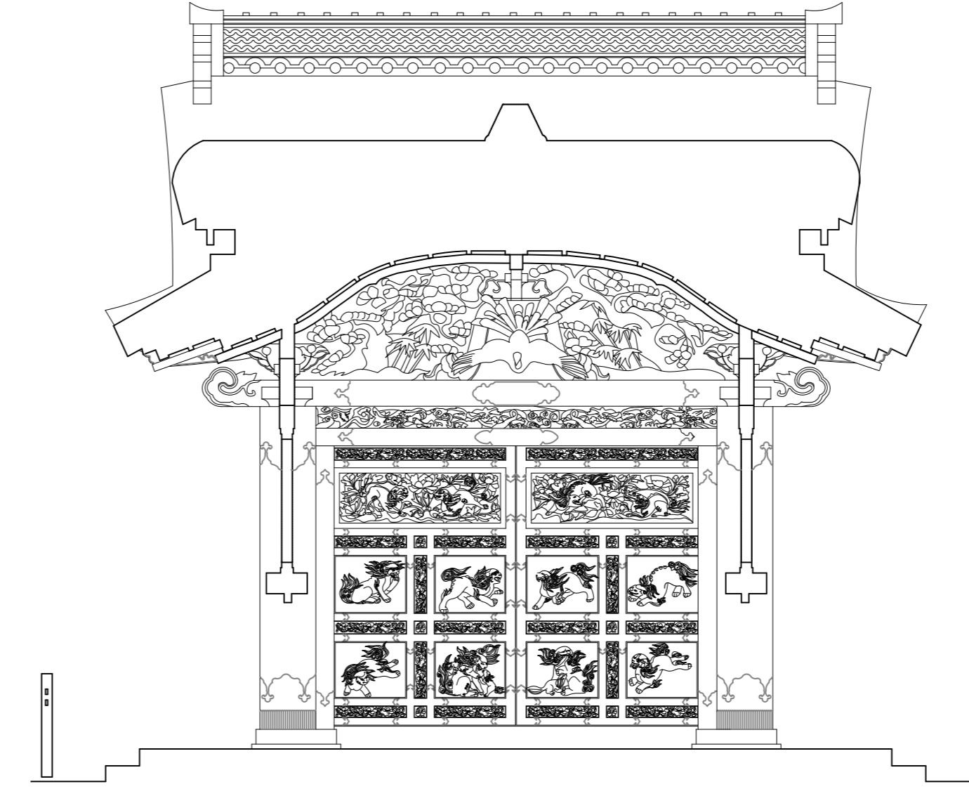
SECTION C-C
