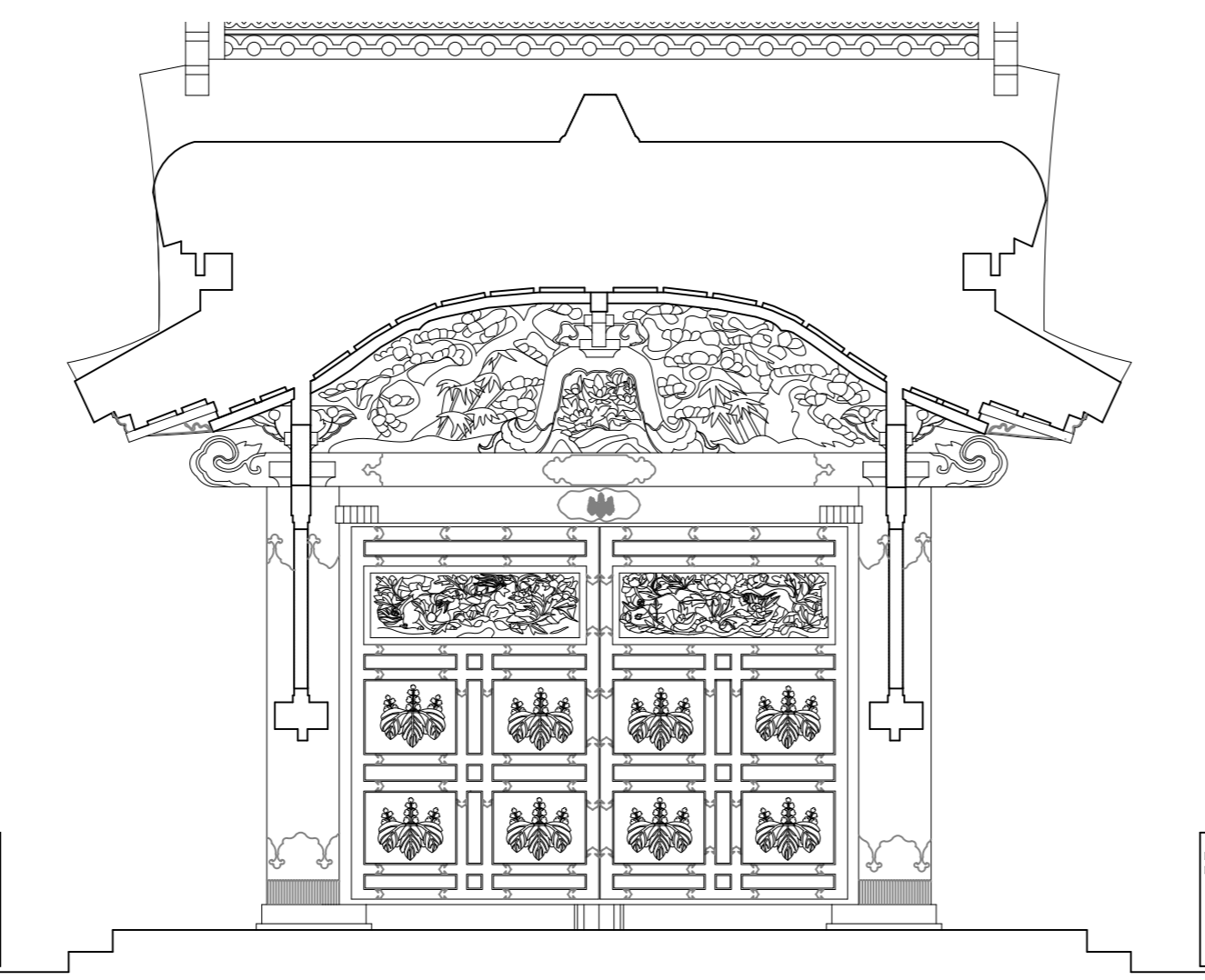
SECTION F-F
