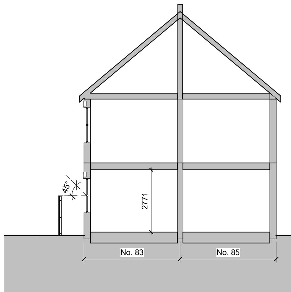
PROPOSED SECTION 1 : 100
