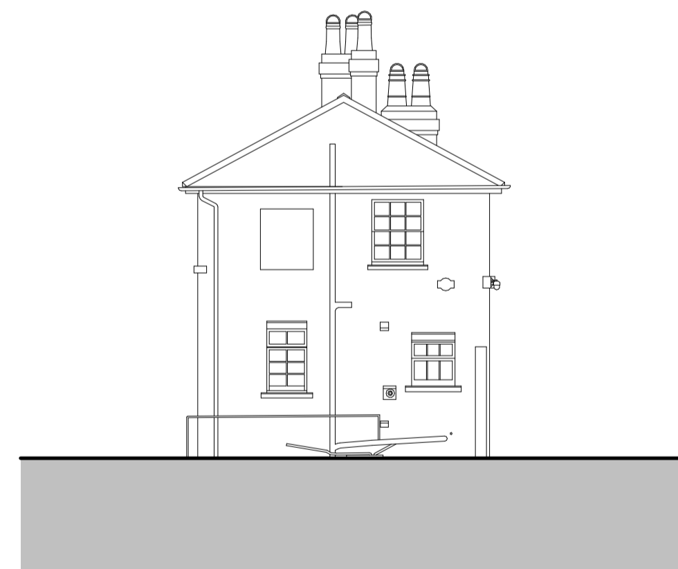
10 Upper Cottage North West Elevation - Existing 1:100
