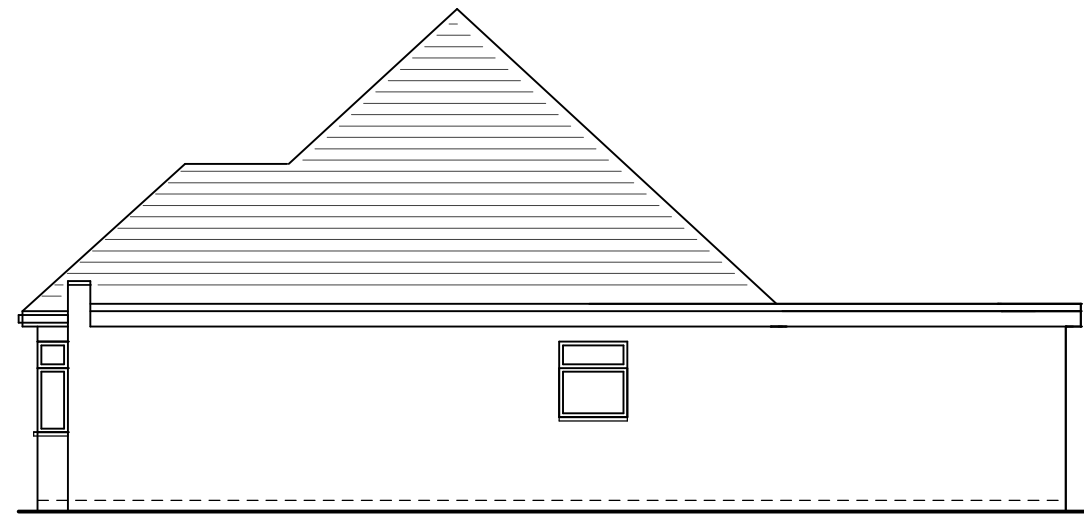
right side (northeast) elevation
