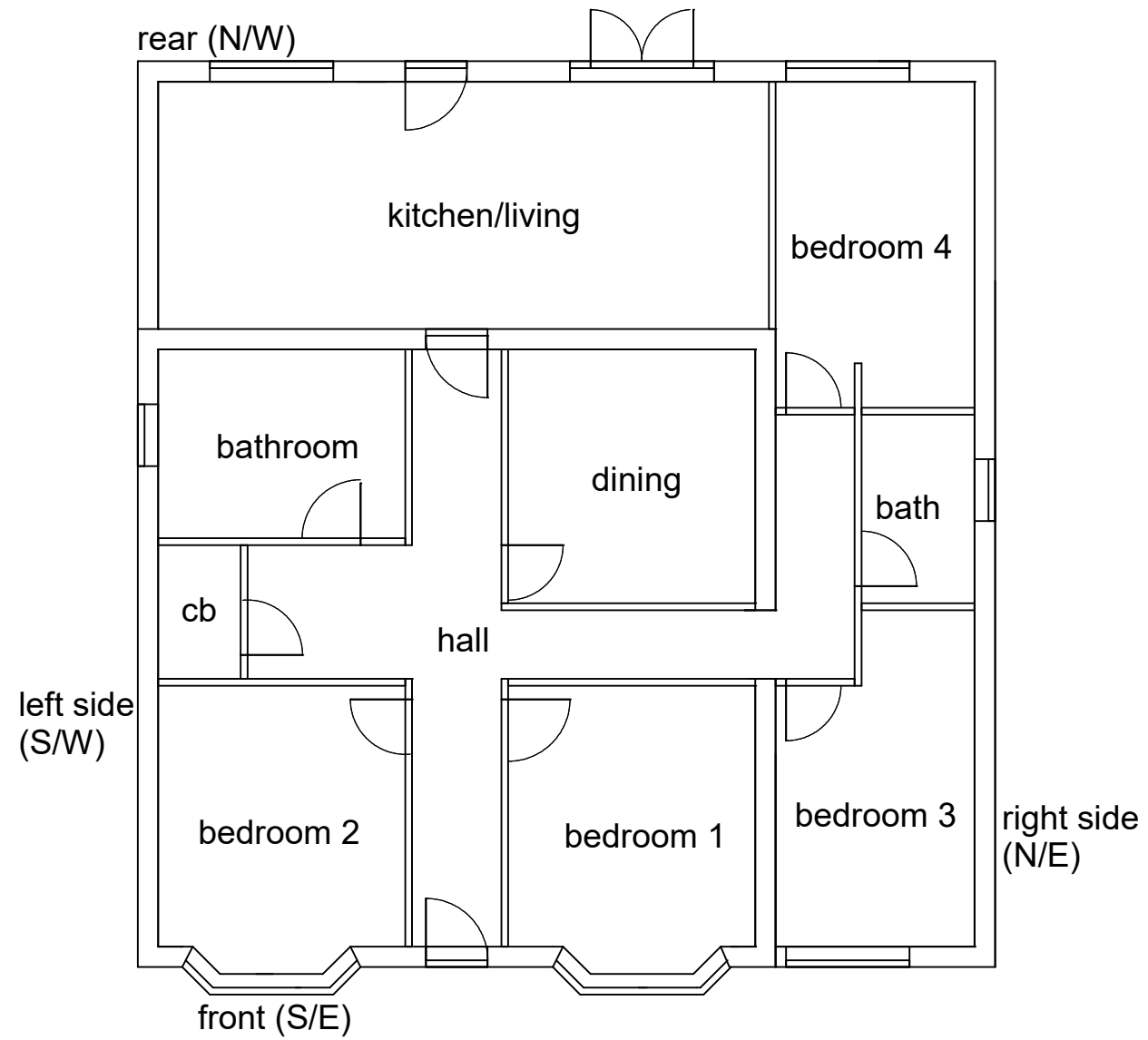
GROUND FLOOR LAYOUT
