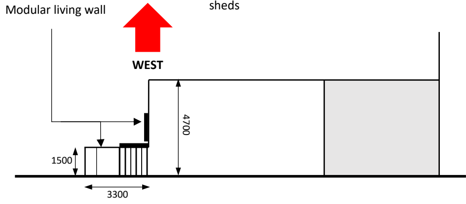
PROPOSED WEST FACING ELEVATION REAR
