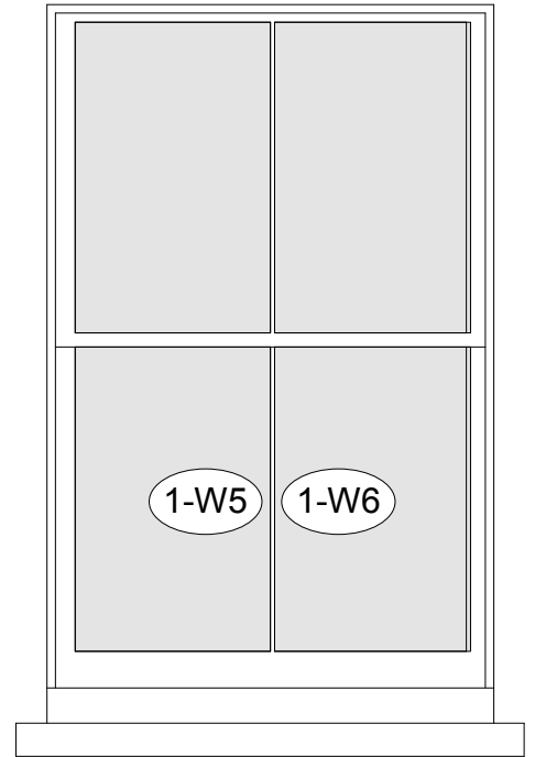
Replacement Timber Vertical Sliding Sash Window to Match Existing
