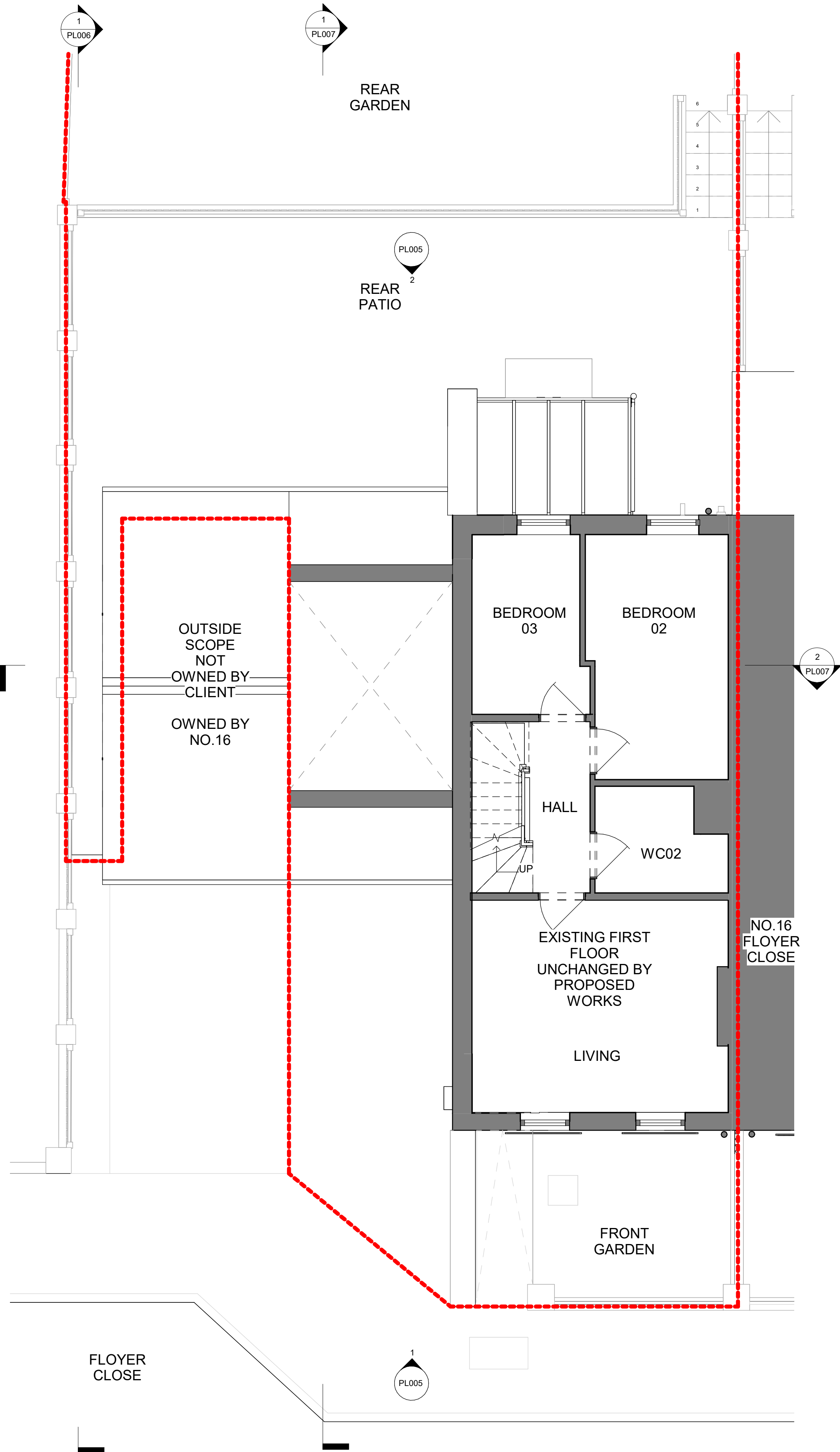
2 Planning - Existing 01 First Floor Plan 1 : 50
