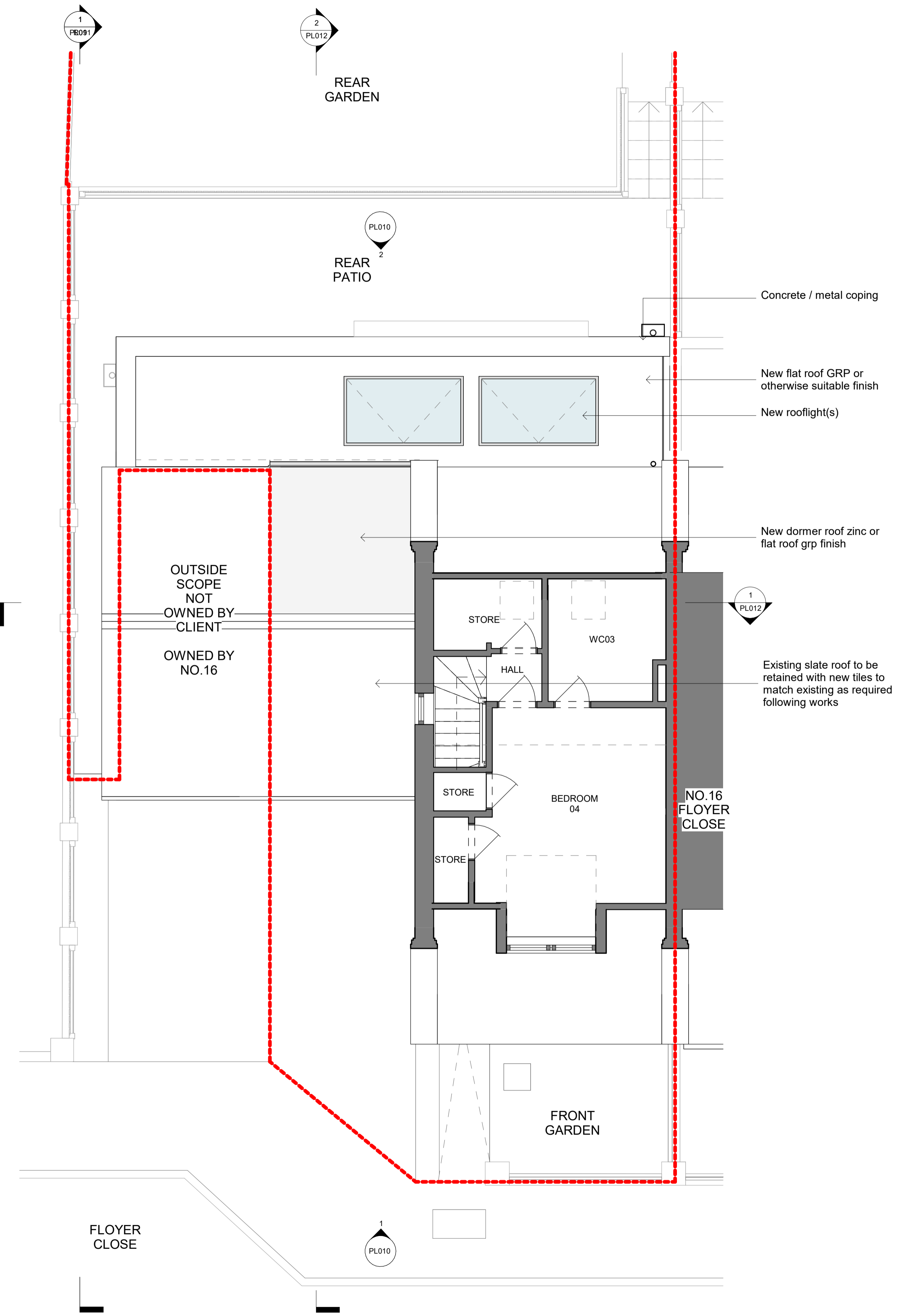
1 Planning - Proposed 02 Second floor plan 1:50
