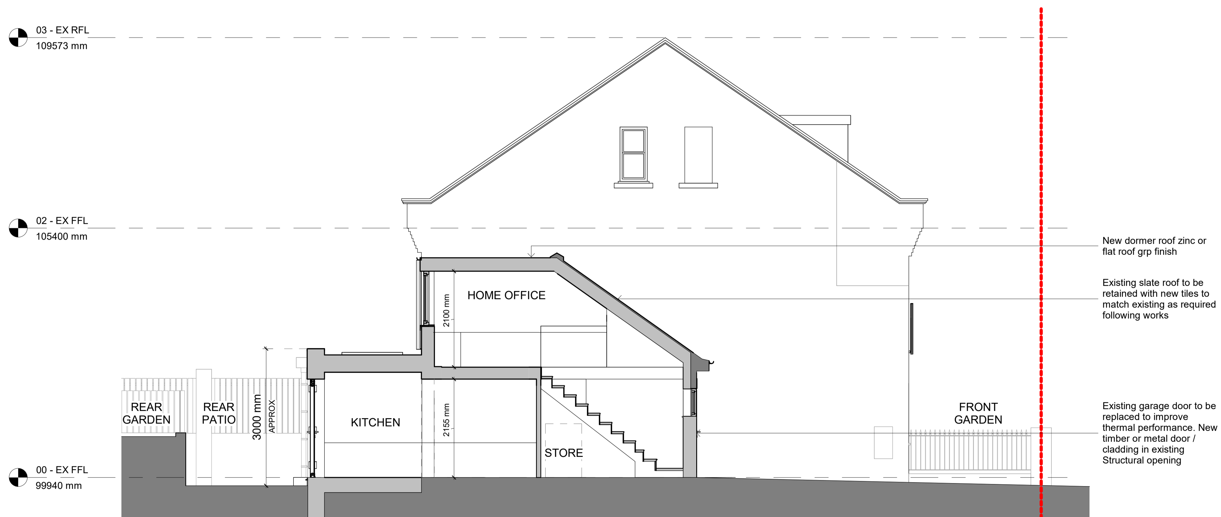
2 Planning - Proposed Longitudinal Section 1:50
