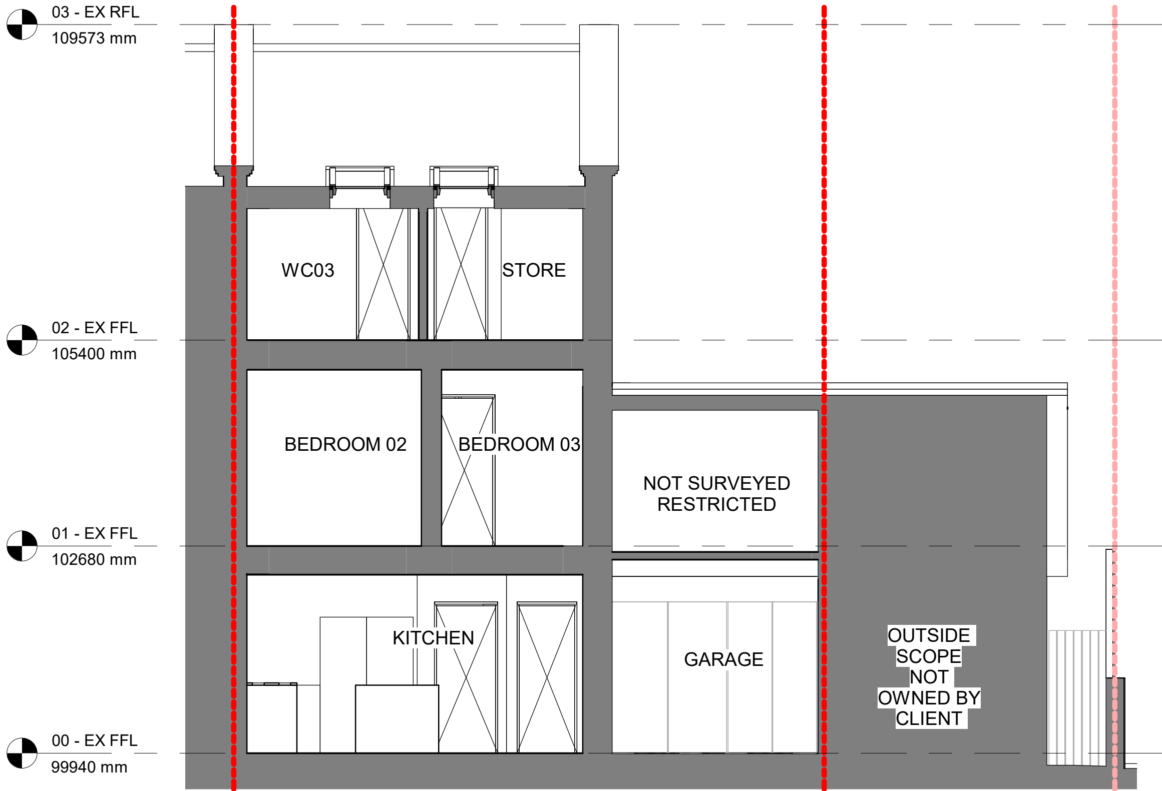
2 | Planning - Existing Cross Section 1 : 50
