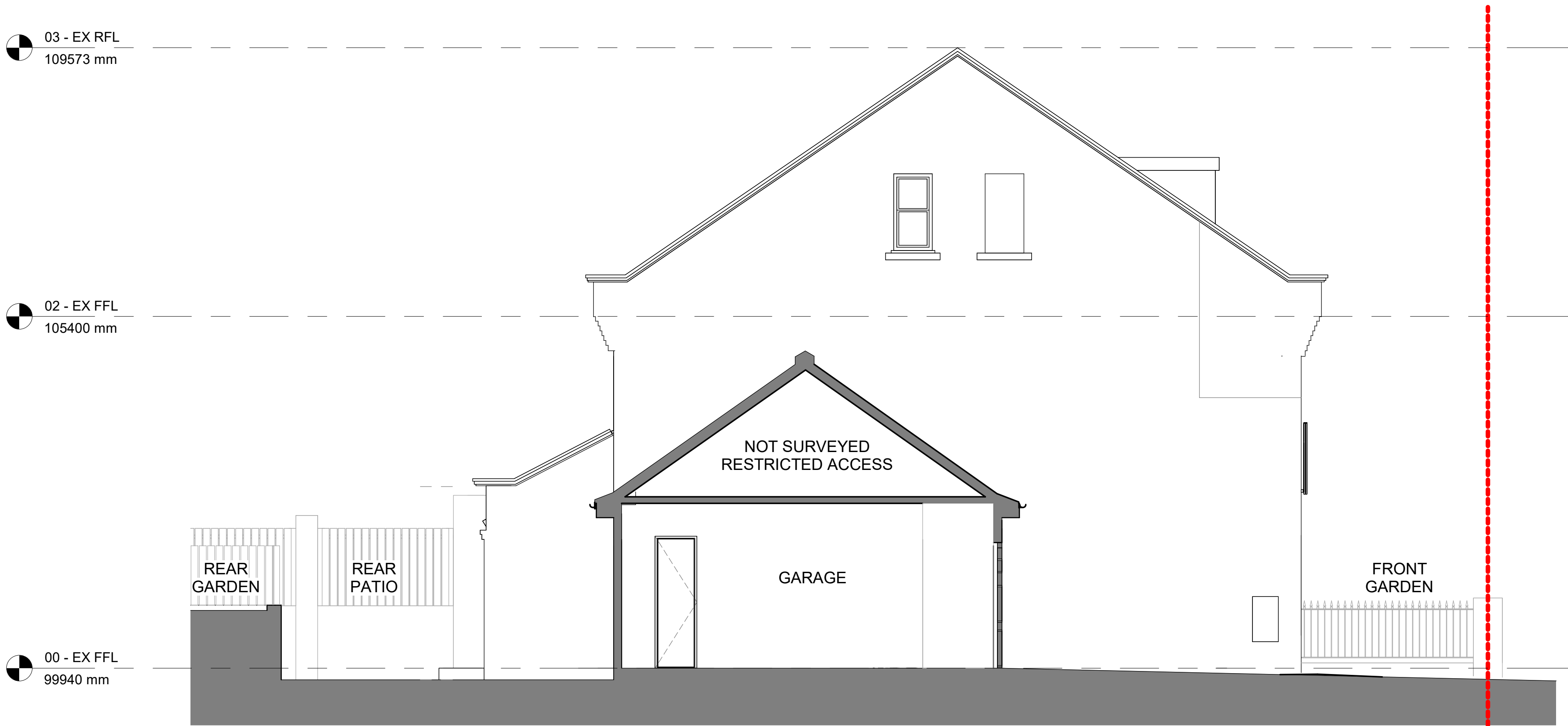
1 | Planning - Existing Longitudinal Section 1 : 50
