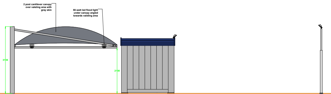
HAND CAR WASH ELEVATION VIEW A
