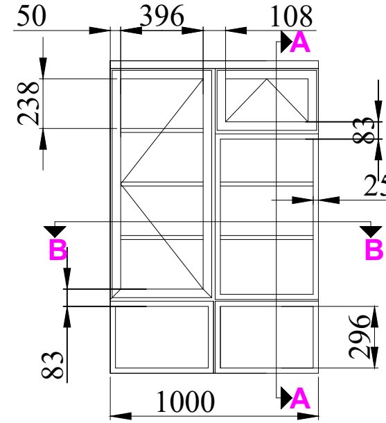
② Proposed Example Type 2 Window Elevation / Section Through
