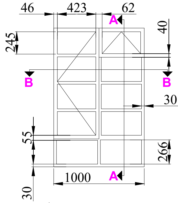
① Existing Example Type 2 Window Elevation / Section Through
