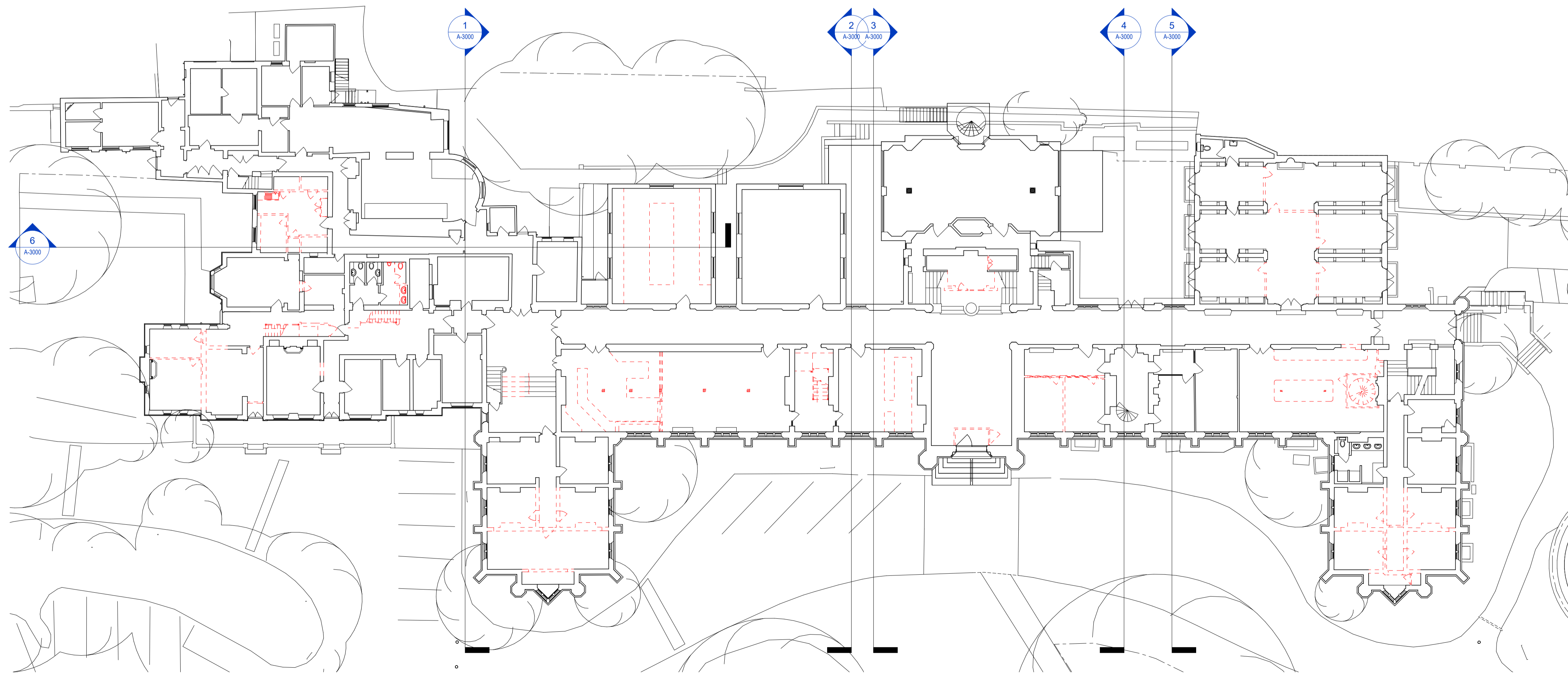
2 Main Building - Ground Floor Existing 1 : 200
