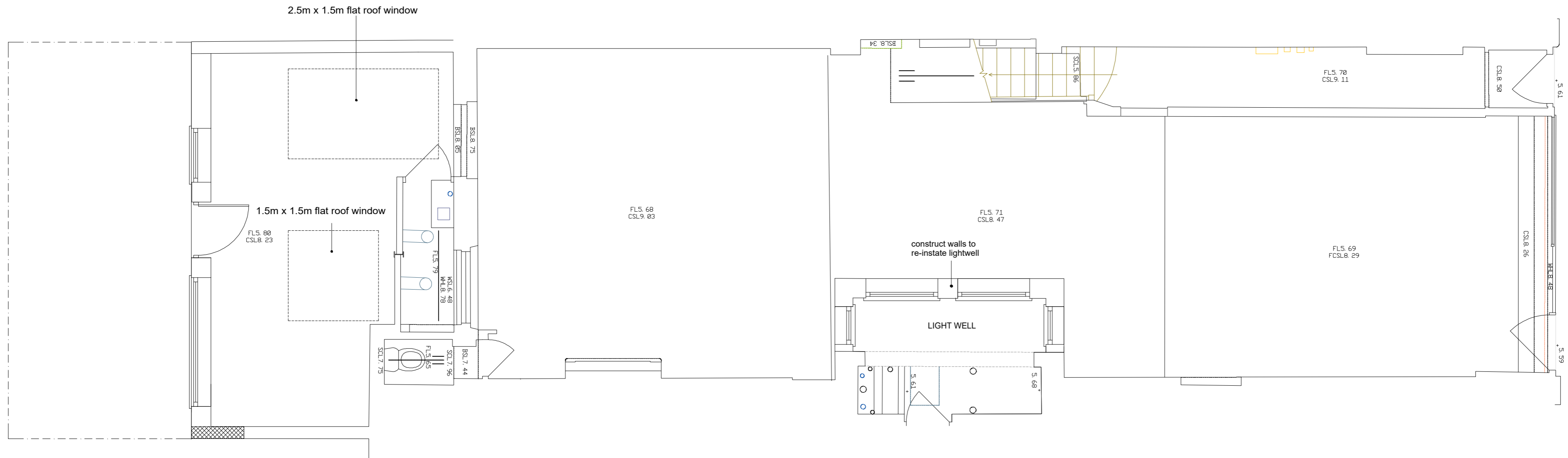
GROUND FLOOR PROPOSED
