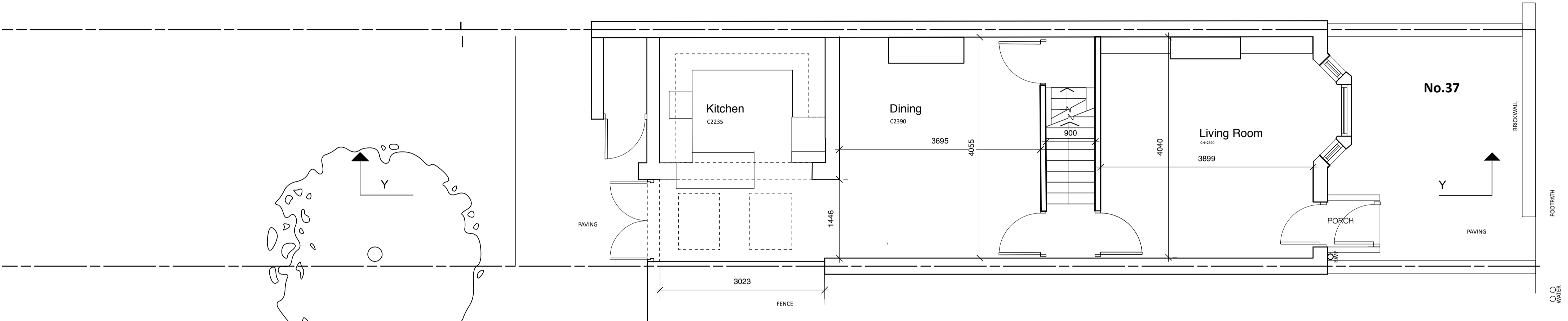
EXISTING GROUND FLOOR PLAN 1:50
