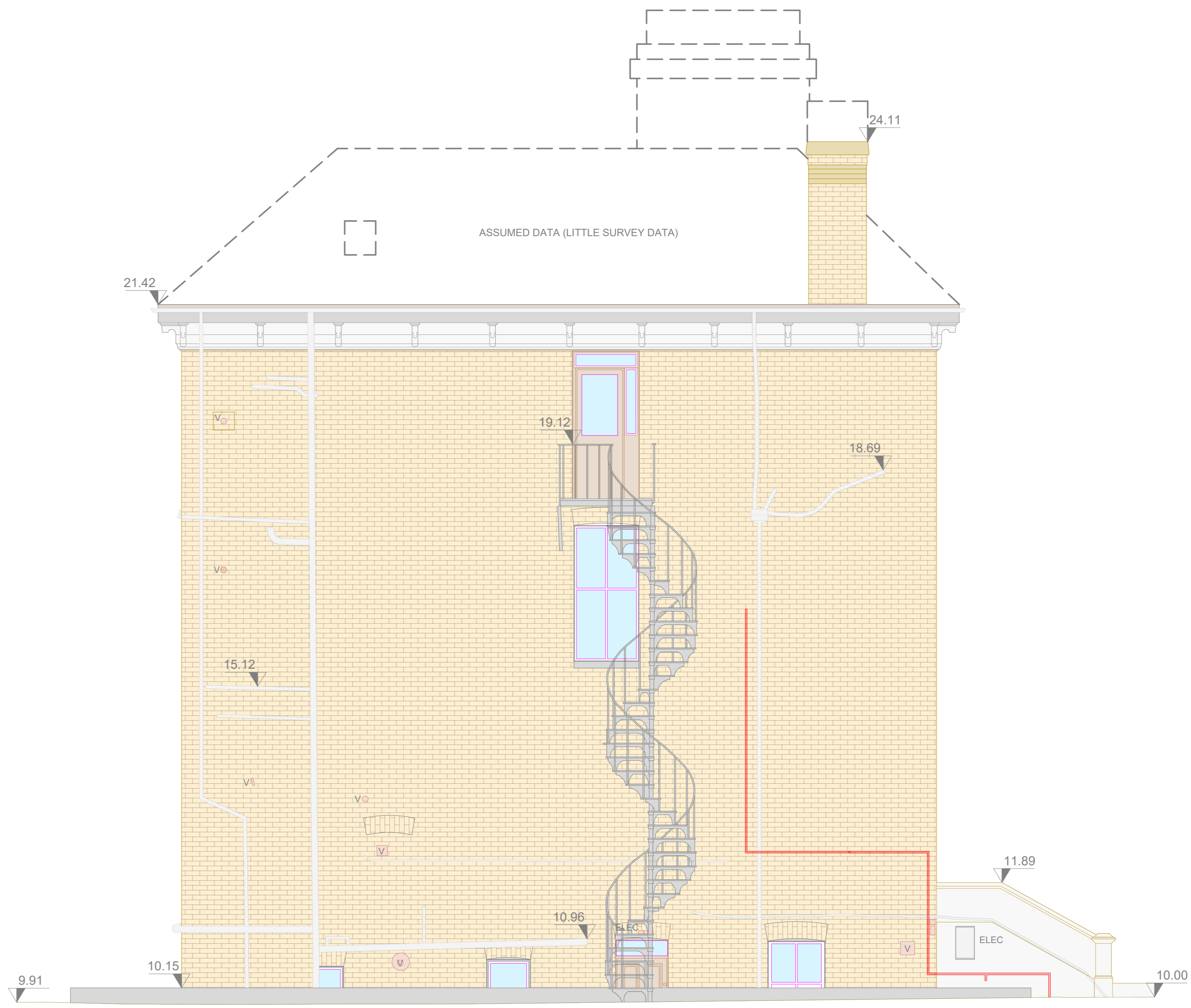
South Proposed Elevation 2nd View
