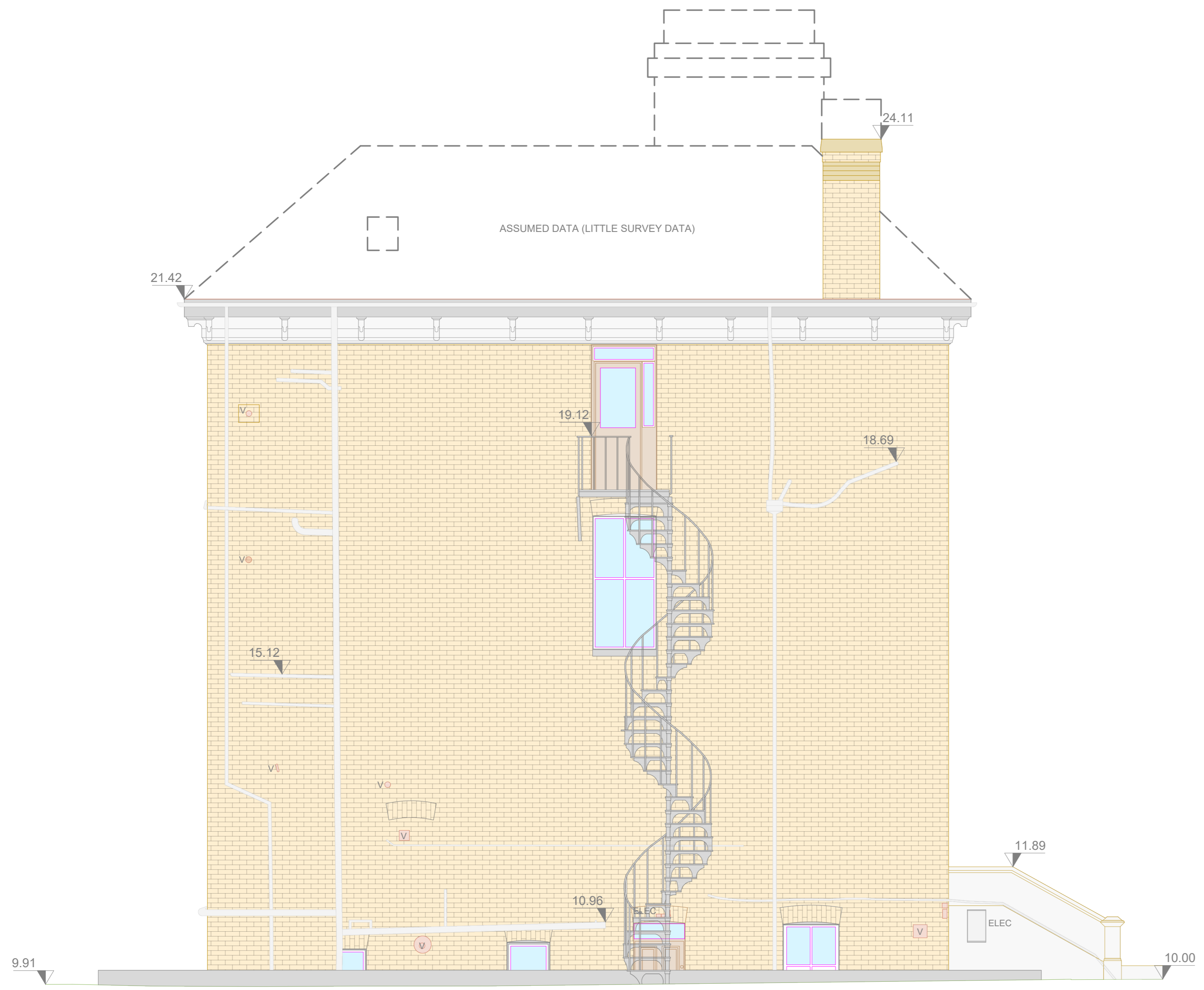
South Proposed Elevation 2nd View
