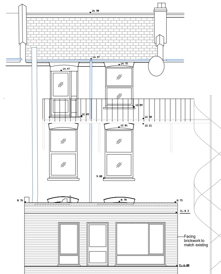
REAR ELEVATION
