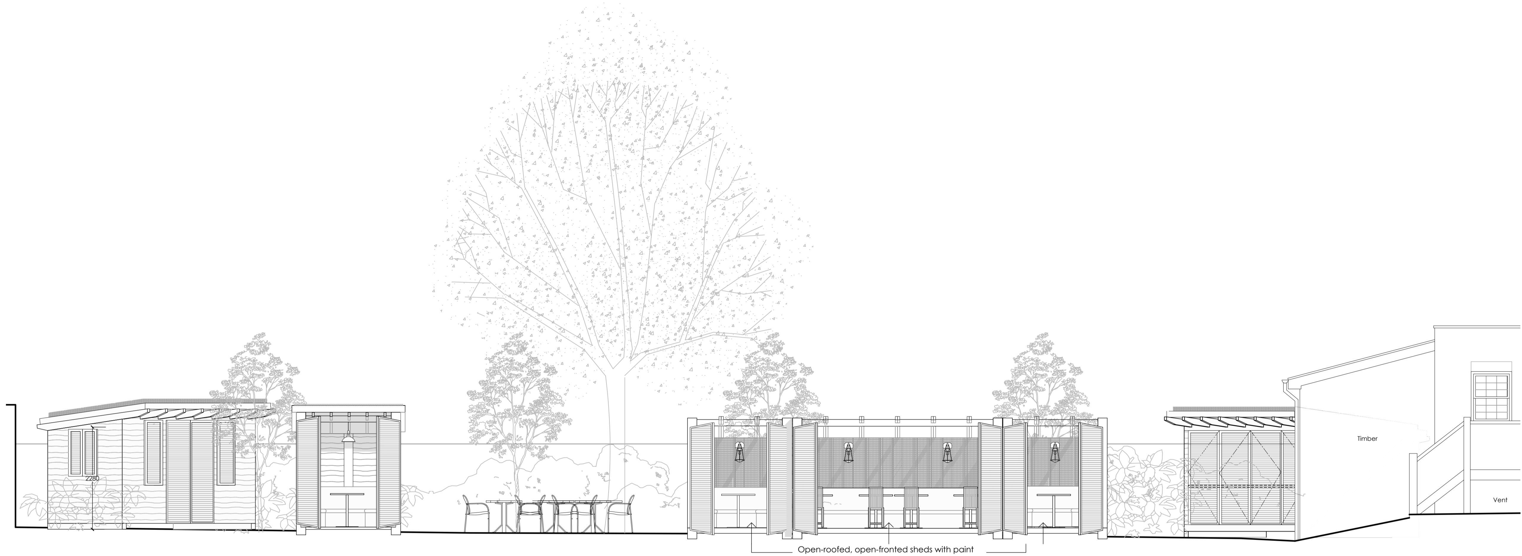
EXISTING ELEVATION A-A Scale 1:50
