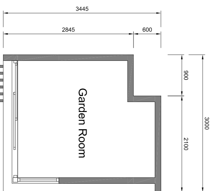
Ground Floor Plan as Proposed - 1:50
