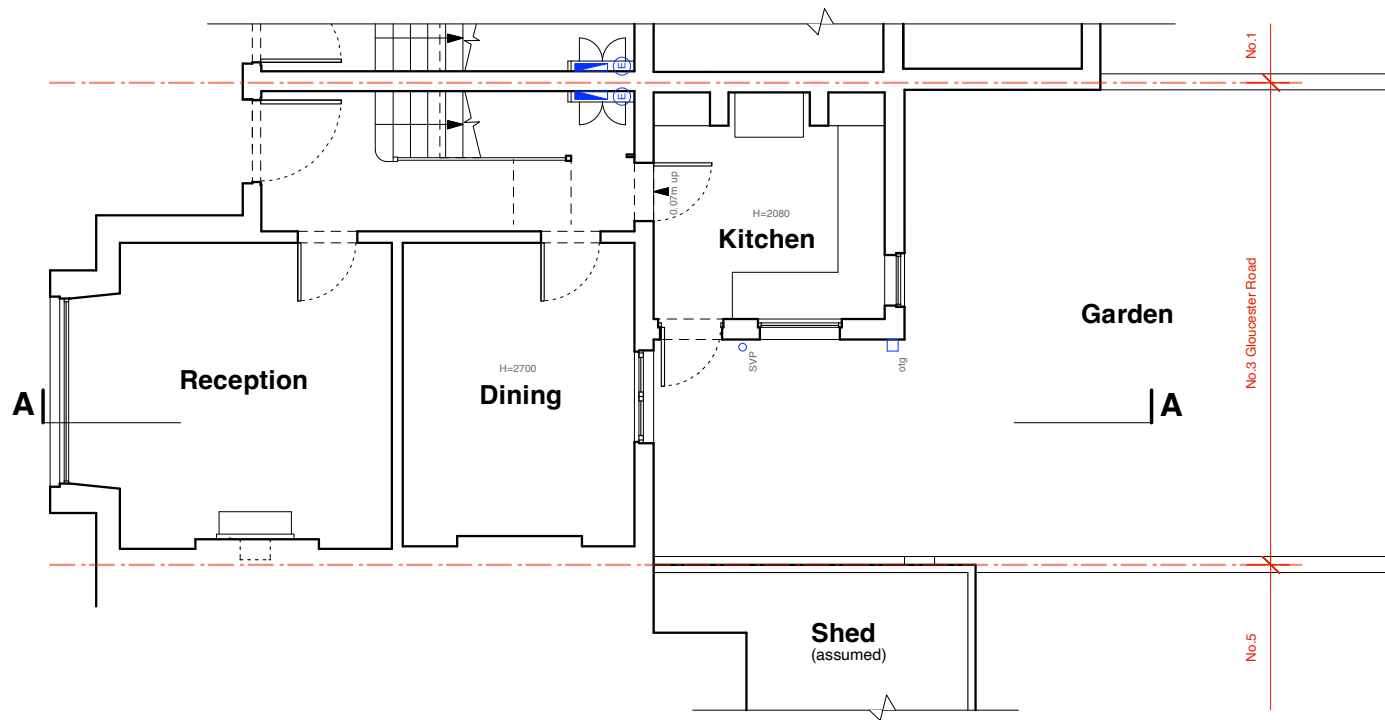
GROUND FLOOR PLAN EXISTING
