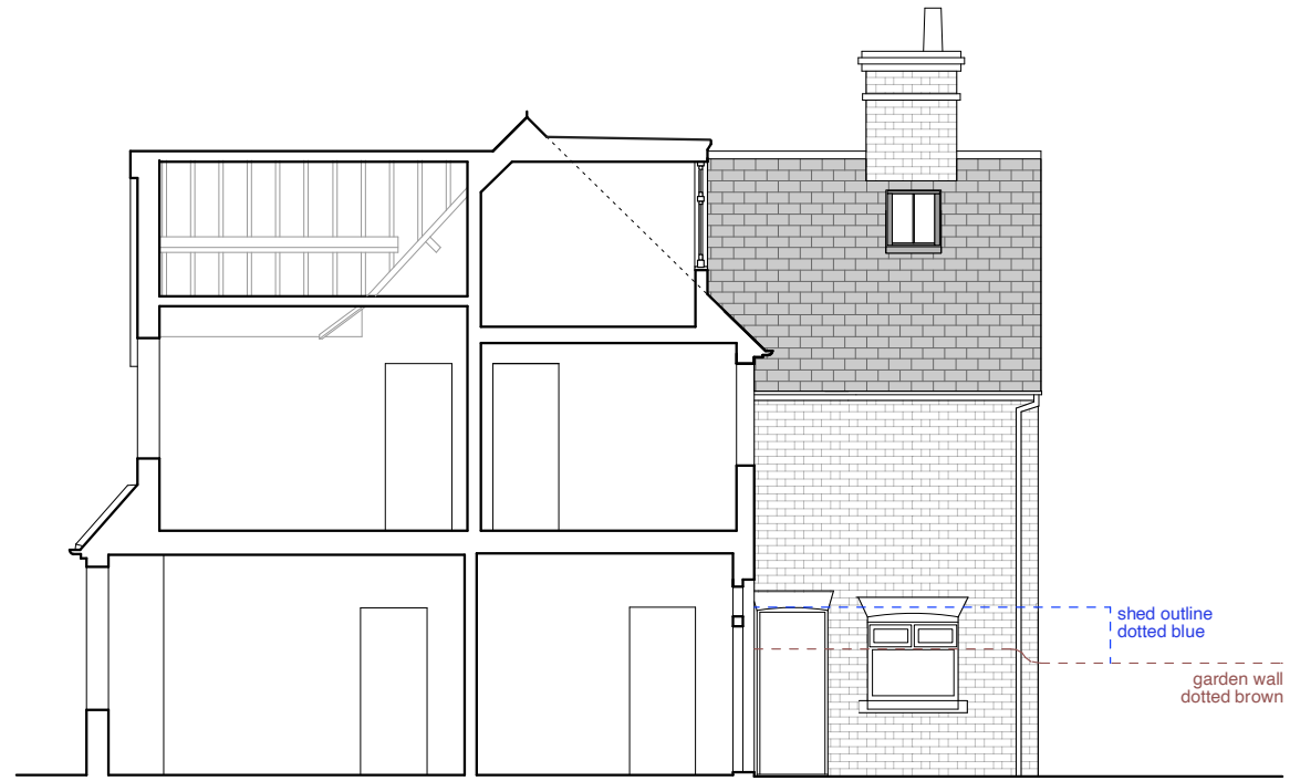
SECTION AA EXISTING
