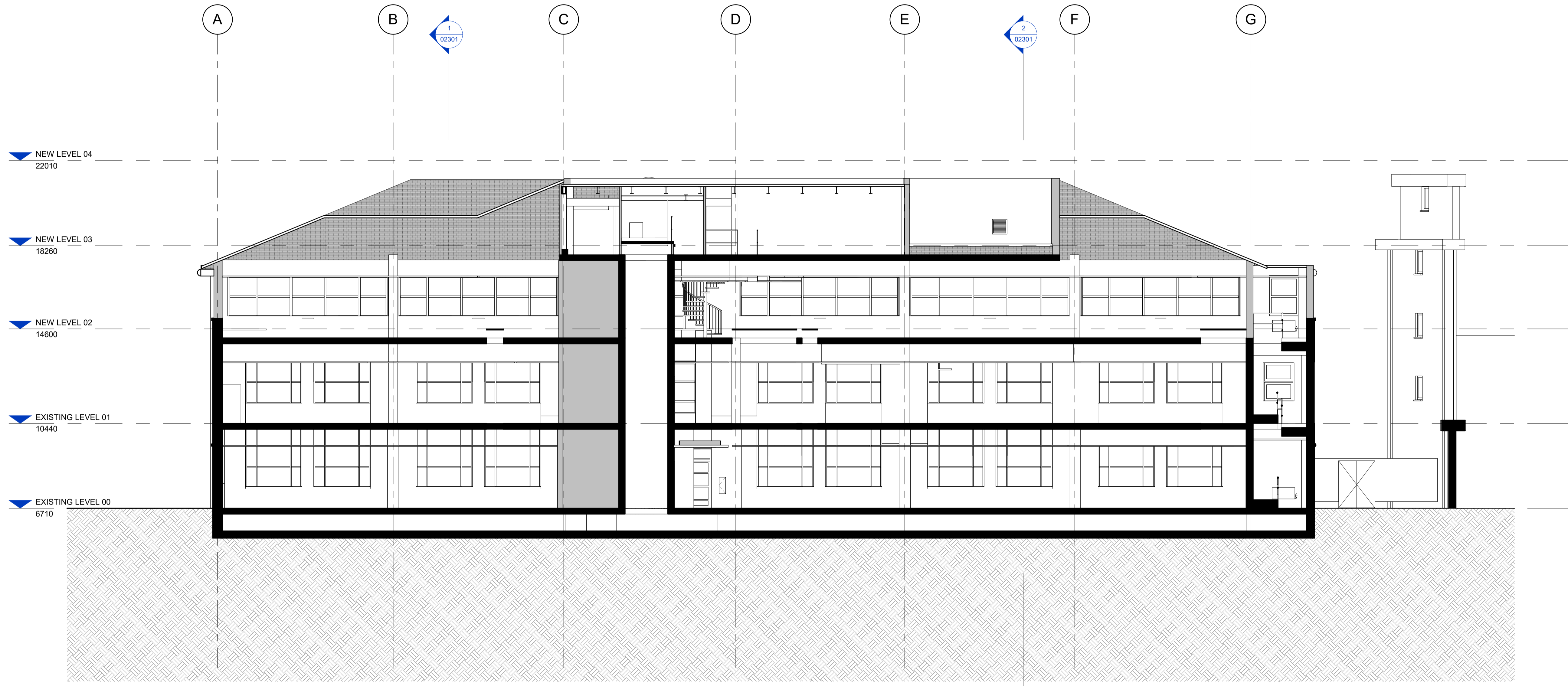
1 Existing Section C-C 1 : 100
